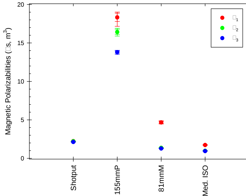
Figure 5-9 – Amplitude variations at 0.089 ms in the derived response coefficients for all items emplaced in the IVS. \beta_1 is in red; \beta_2 is in green; and \beta_3 is in blue.
