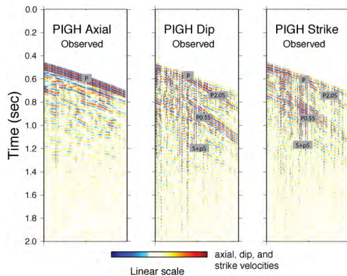
Figure 2. Observed three-component waveforms from the downhole array for a chemical shot located at PASO station PIGH. Seismograms are low-pass filtered at 0.023 s (43.5 Hz).
