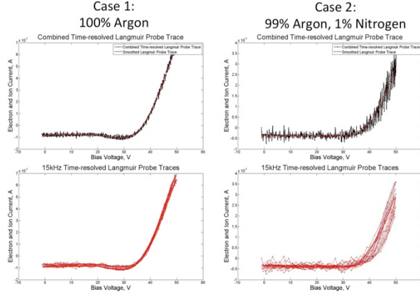
Fig. 4: Time-resolved Langmuir probe (LP) traces.
