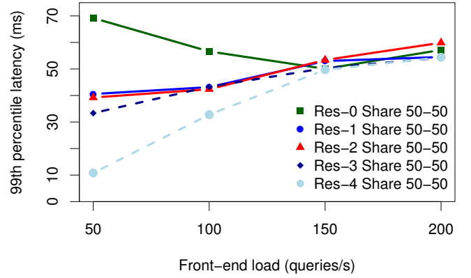
Figure 8: When the front-end client is sending low throughput, reservations are an effective way of reducing queue time at HDFS. Proportional share is insufficient because it will run batch requests when the front-end queue at HDFS is empty, forcing newly arriving front-end requests to wait in the queue.
