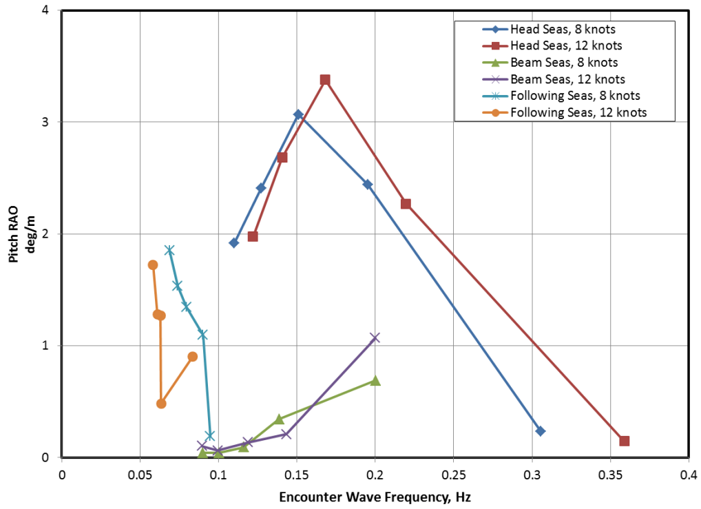
Figure 27. Regular wave pitch RAOs for all headings and speeds, 1/60 wave steepness.
