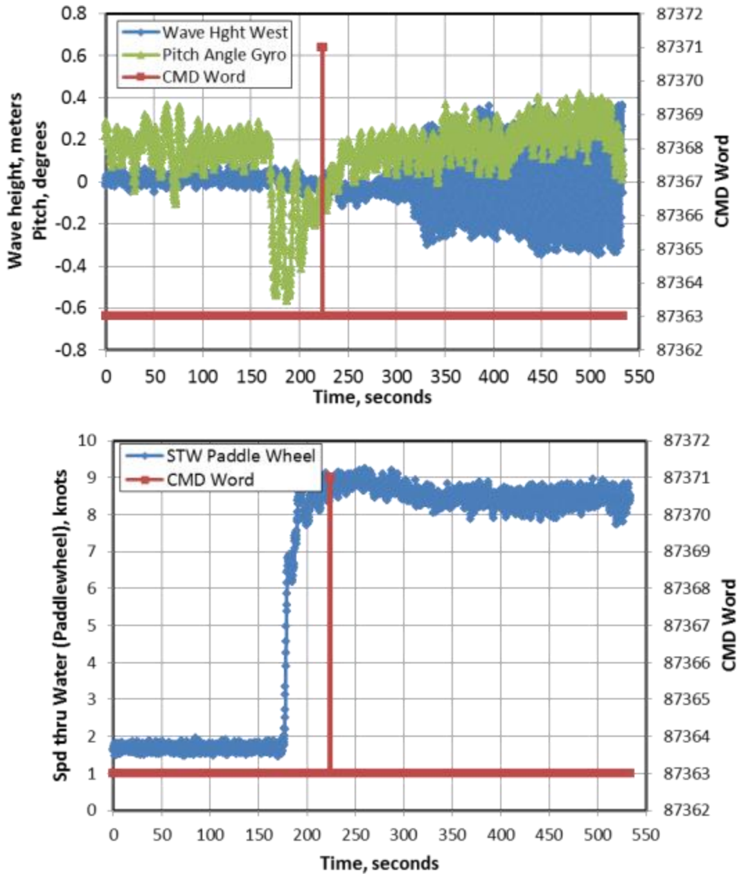
Figure 25. Example data from a regular waves transient run.
