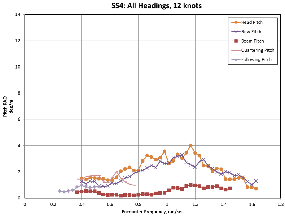
Figure D8. Pitch RAOs, SS4, all headings, 12 knots.
