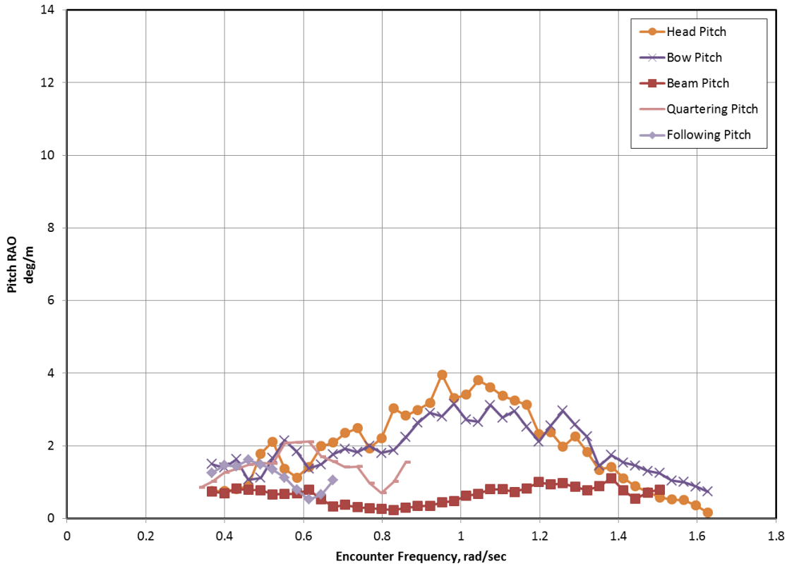
Figure 30. Pitch RAOs for SS3, all headings, 8 knots.
