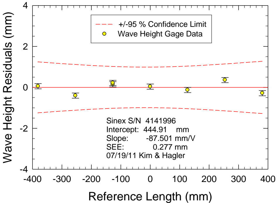
Figure A13. MASK Bridge Probe BP1 Calibration
