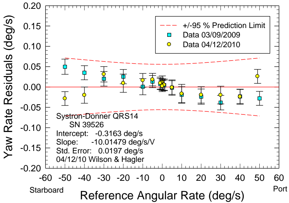
c. Yaw Rate
