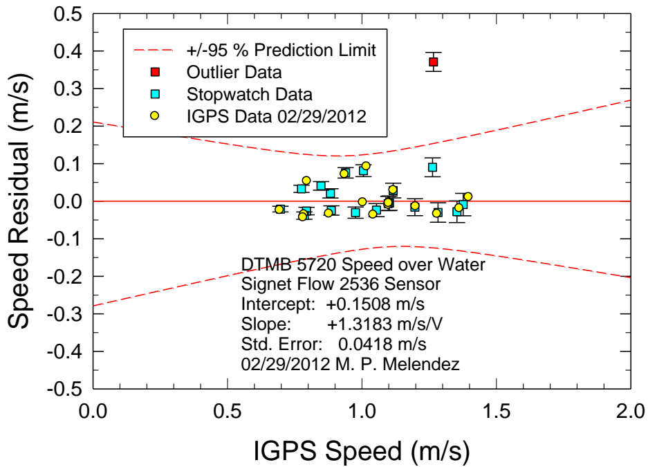
a. Calibration by Stopwatch
