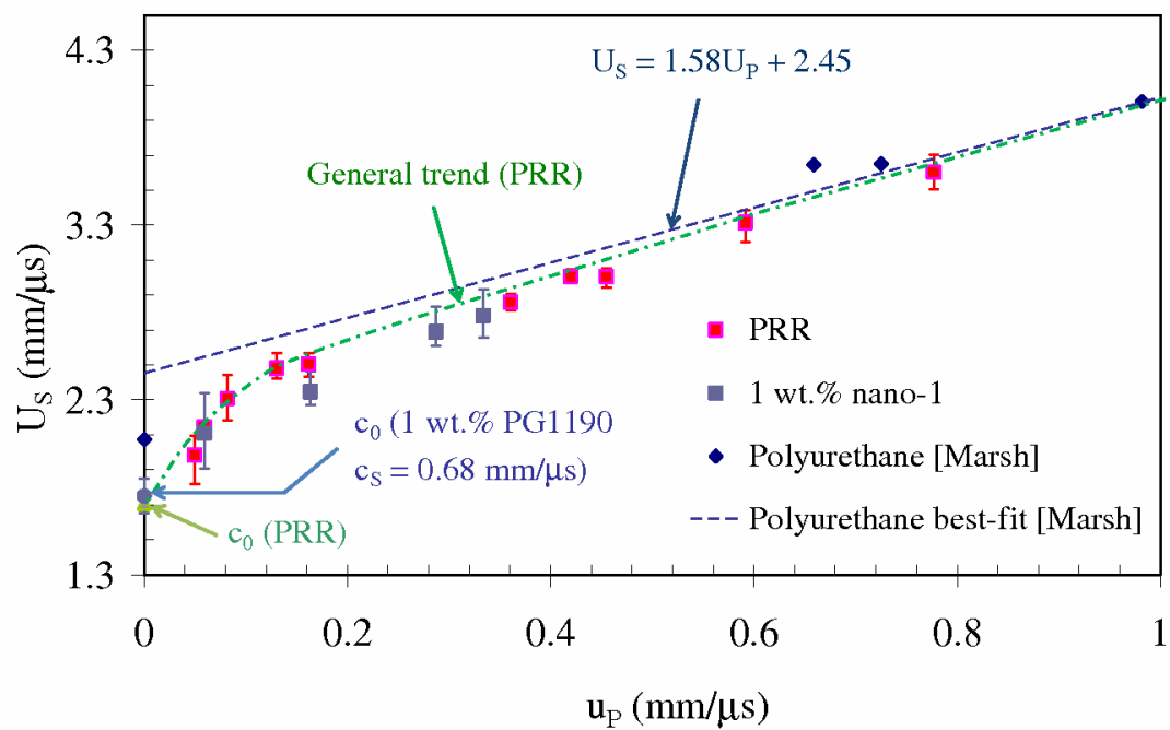
Figure 2.6: U_s - u_p Hugoniot for pure and 1 wt.% PG1190 Polyurethane Replacement Resin (PRR) - adapted with permission from [25]. Comparative data is taken from [30]
