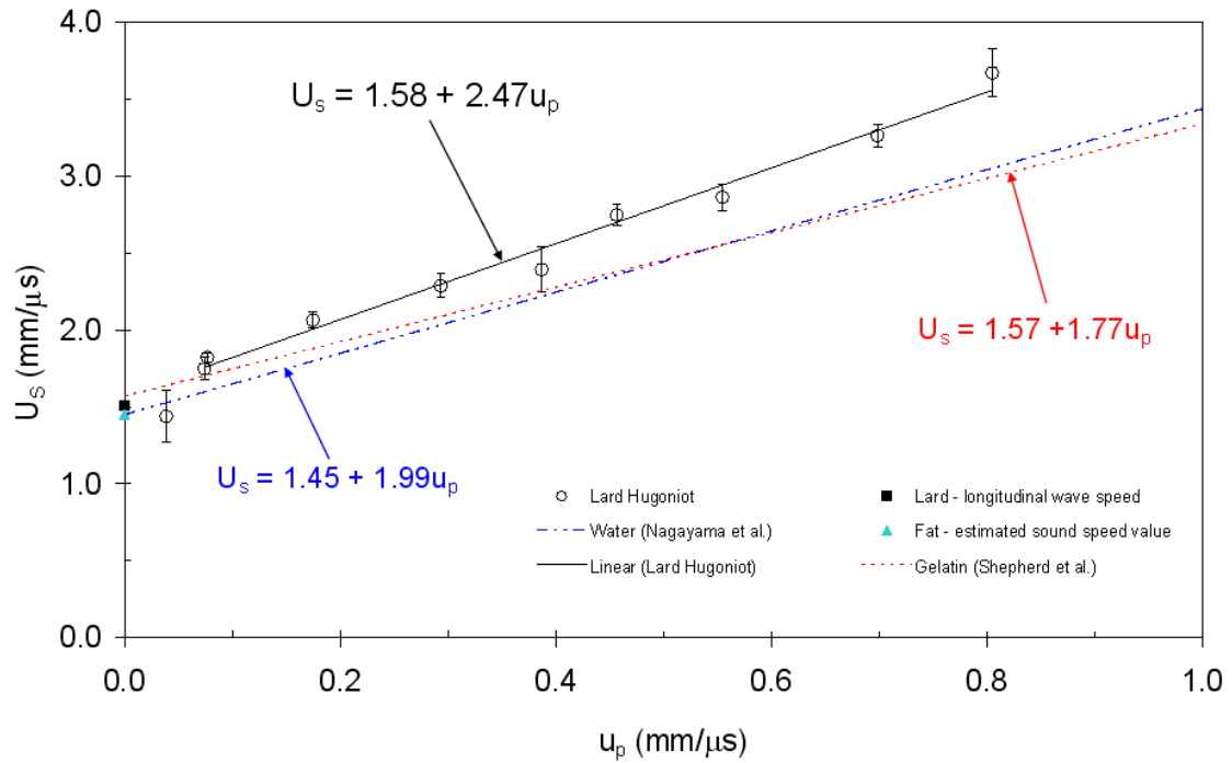
Figure 8.2: Principal ( U_s - u_p ) Hugoniot of the adipose material
