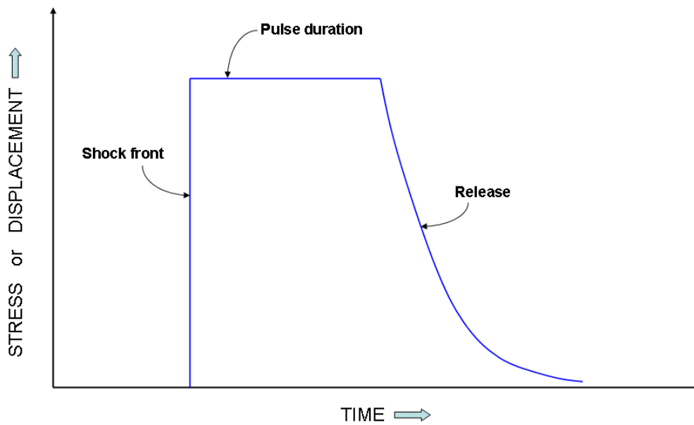
Figure 2.7: Idealised shock wave profile [19]
