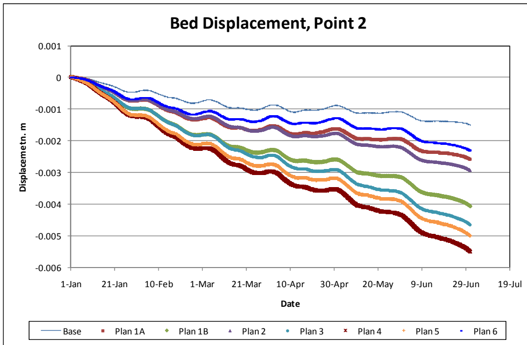
Figure 6-51. Cumulative bed displacement for Point 2.
