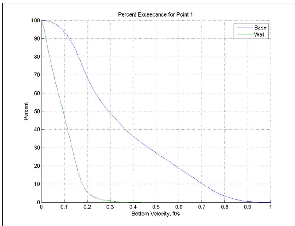
Figure 7-26. CDF curves for the Base and Wall plans at Point 1.
