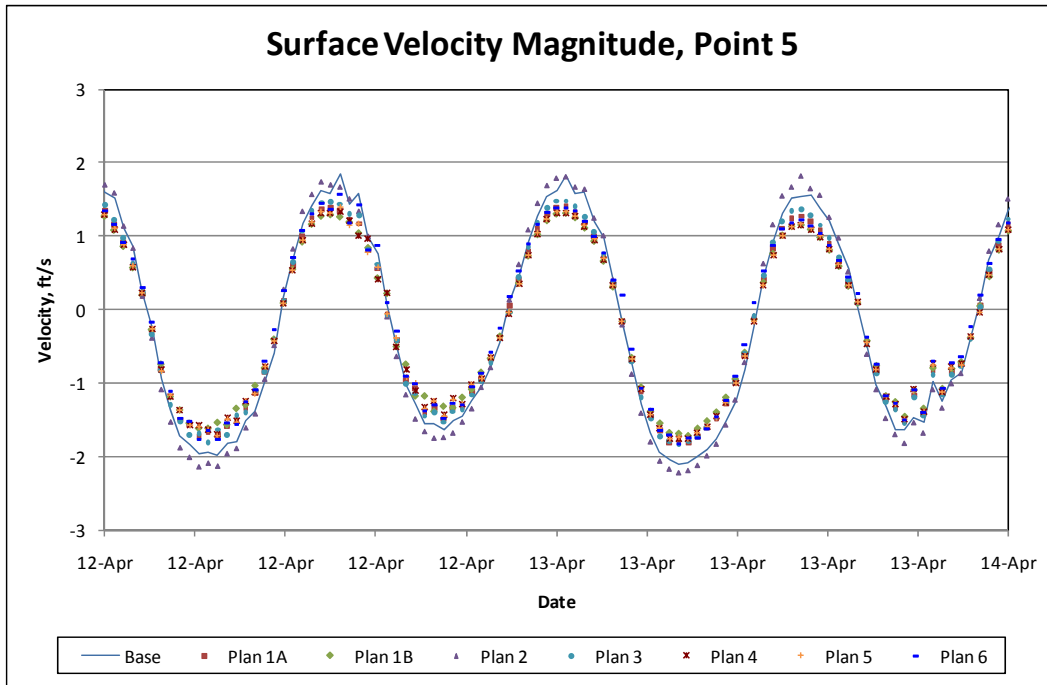
Figure 6-18. Surface velocity at Point 5.
