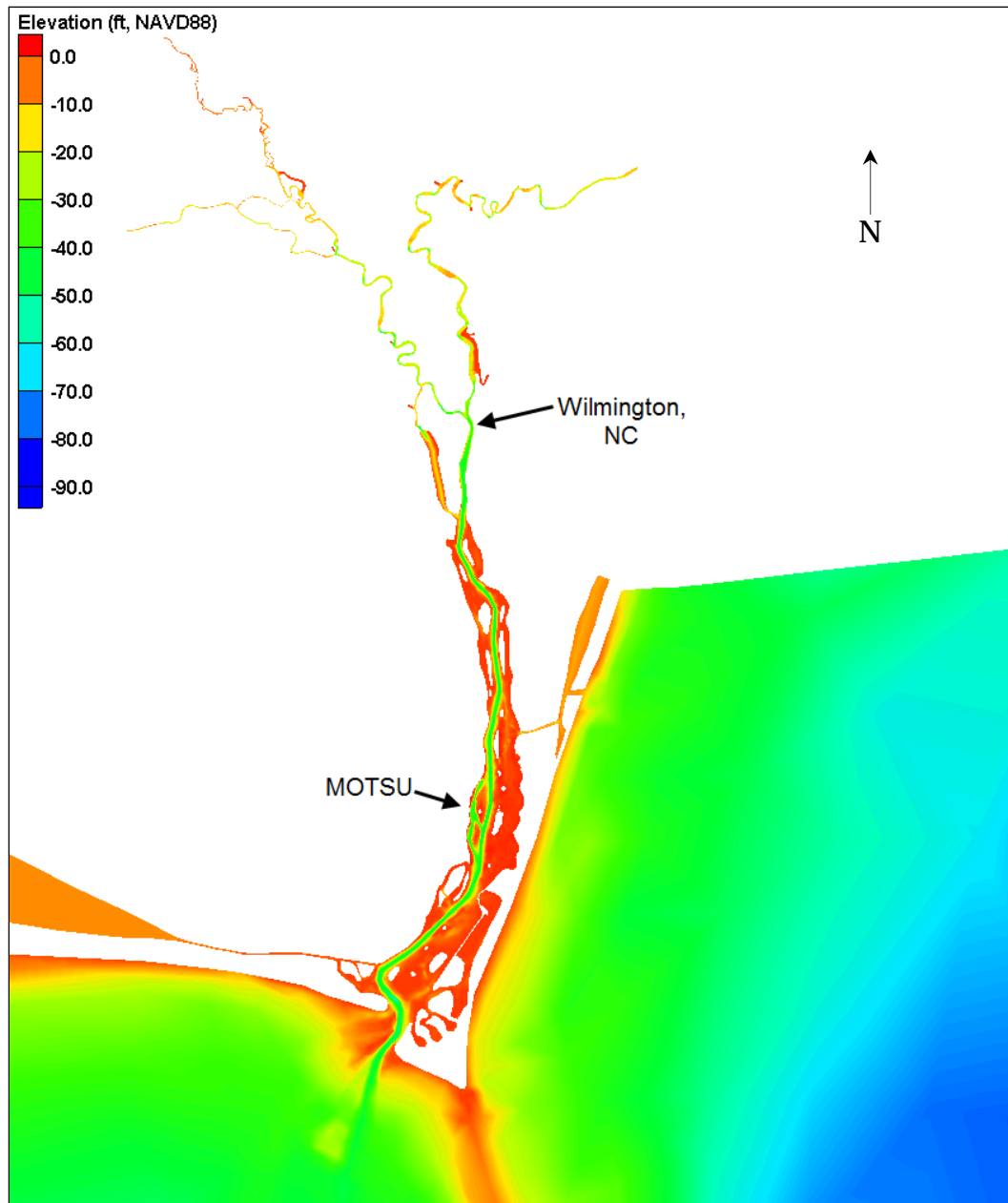
Figure 4-5. Mesh bathymetry.
