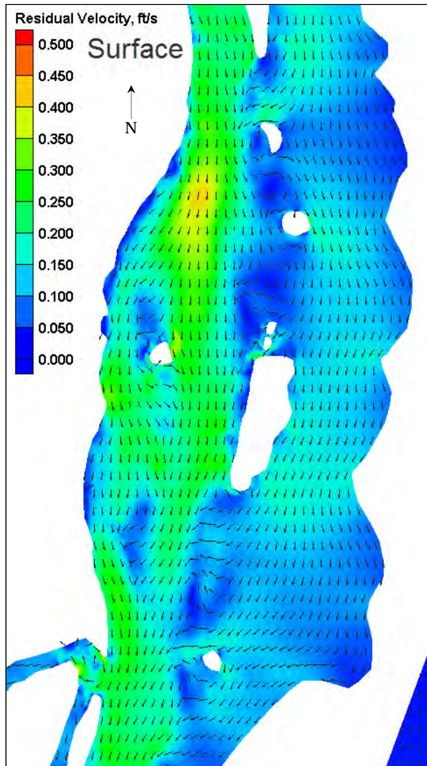
Figure 6-42. Six-month surface velocity residual.
