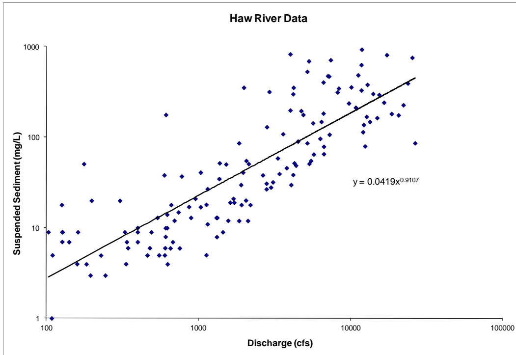
Figure 4-15. Haw River sediment load rating curve (100 mg/L = 1 ppt).
