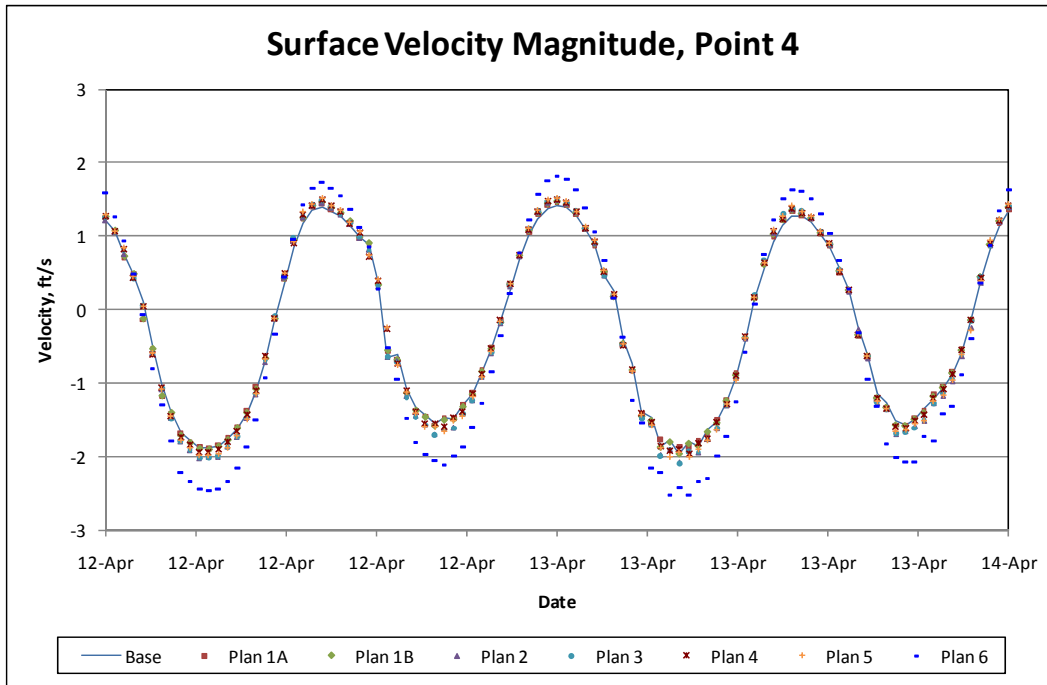
Figure 6-16. Surface velocity at Point 4.
