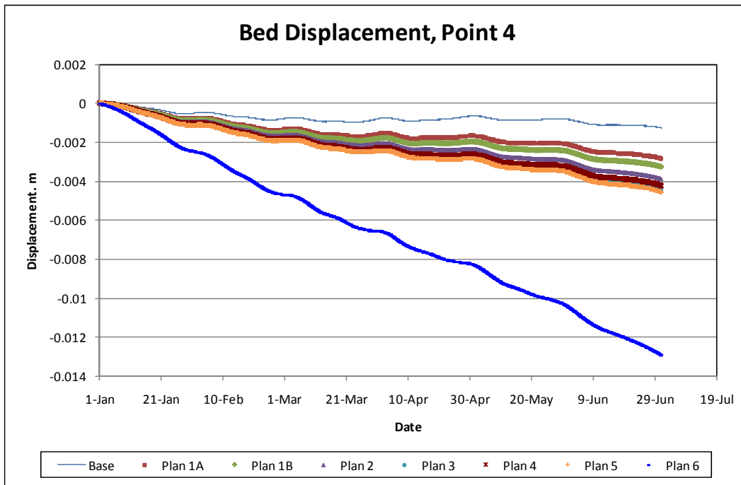
Figure 6-59. Cumulative bed displacement for Point 4.
