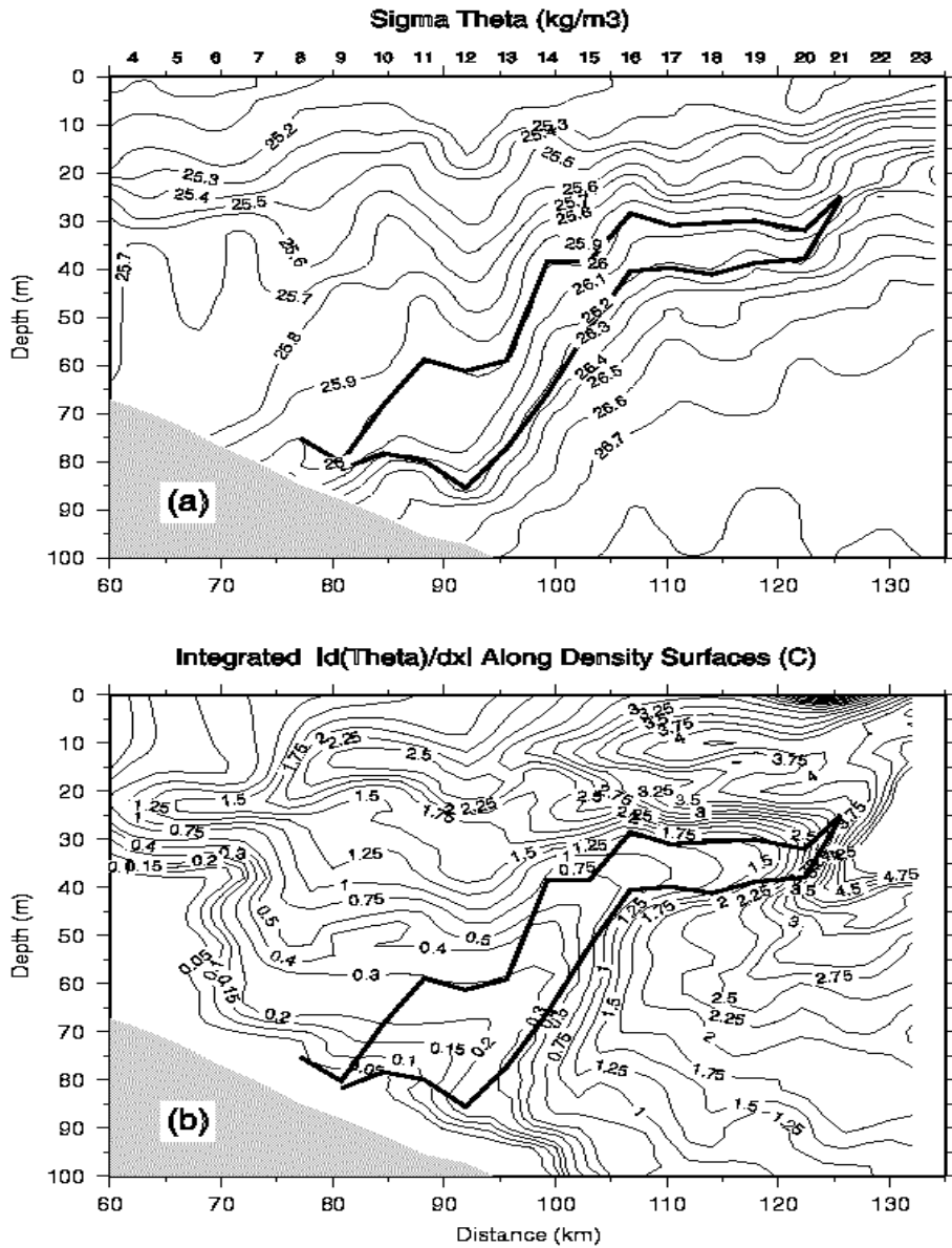
Figure 1: (a) Potential density of the shelfbreak front. The thick lines denote the detached BBL as revealed by a minimum in stratification. (b) Integral of \int Id(\Theta)/dxl along density surfaces, starting from the inshore side of the section. The tongue of low values also reveals the separated BBL.
