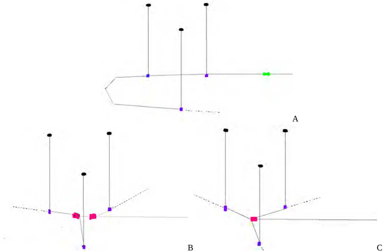
• Figure 7. Three alternate hydrophone layouts using a modular approach. A) Linear layout with triplet connected to trunk cable with connector (green). B) Layout utilizing two branching units (red). C) Layout using single branching unit. (Figures from [Mallin, 2012])
