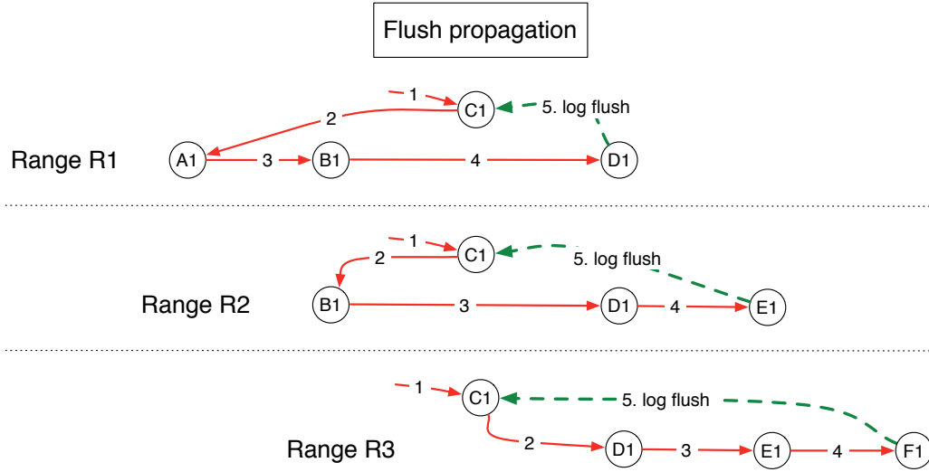
Figure 2.11: Phase 2 of Join: Flush. The Flush protocol ensures that a new node can join R chains at appropriate locations while maintaining strong consistency, and does so with minimal blocking. The Flush message for the case where the new node joins as the head, Range R3 in the example above, also has a flag indicating that D1 , E1 , and F1 can split the range from B1-D1 into B1-C1 and C1-D1 .
