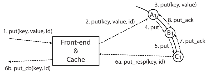
Figure 2.7: Lifecycle of a put with chain replication—puts go to the head and are propagated through the chain. Gets go directly to the tail.
