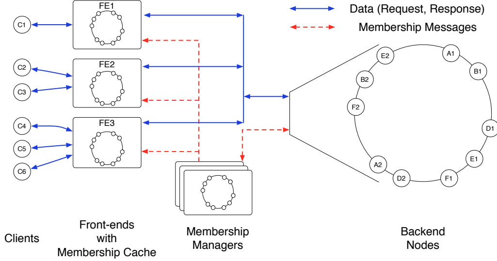
Figure 2.1: FAWN-KV Architecture.
