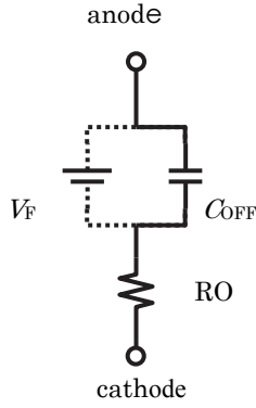
Fig. 3.9 Diode model used for analytical analysis. Dotted line indicates ON state path where current flows against the fixed voltage of V_F .
