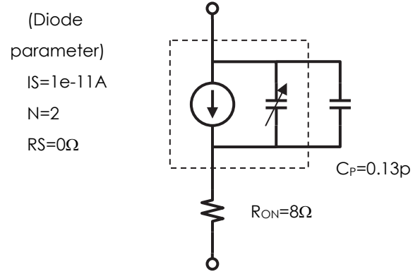
Fig. 3.3 Diode model used in circuit simulation. CP and RON placed out of the intrinsic diode model.
