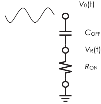
Fig. 3.11 Model for OFF state loss calculation. Sinusoidal wave which amplitude is V_{DC} + V_F is applied on the series connection of C_{OFF} and R_{ON} .
