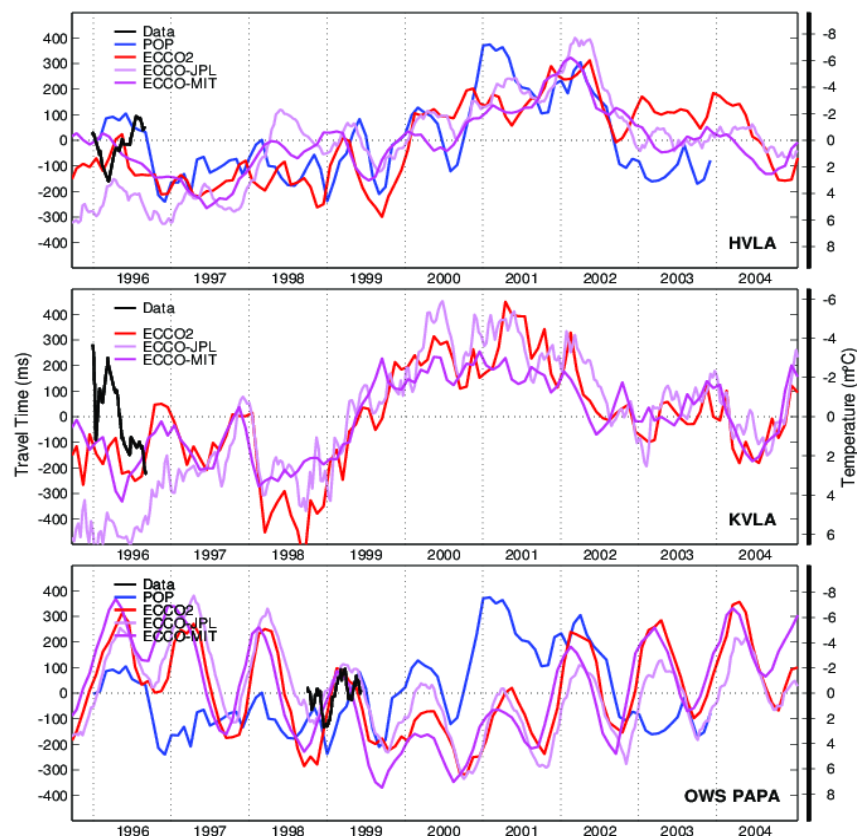
Figure 3 Travel time time series over a decade derived from several ocean models or state estimates for the three acoustic paths: Pioneer to KVLA, Pioneer to HVLA, and Kauai to OWSP. The state estimates agree generally, but differ substantially in detail. The black lines in each panel are time series measured during the ATOC program. To obtain travel times associated with measured arrivals, the time mean state of some models require correcting.
