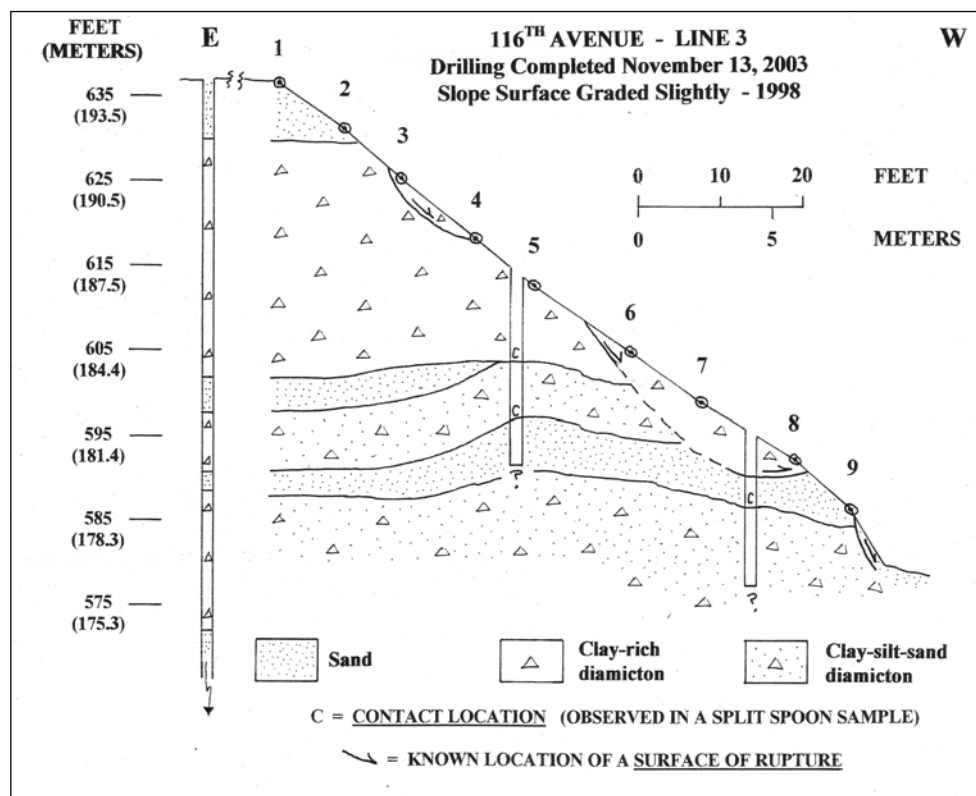
Figure 32. 116th Avenue cross sections for Survey Lines 2 and 3. Sections modified after drilling borings for instrumentation and wells (cross sections drawn by Ronald B. Chase).
