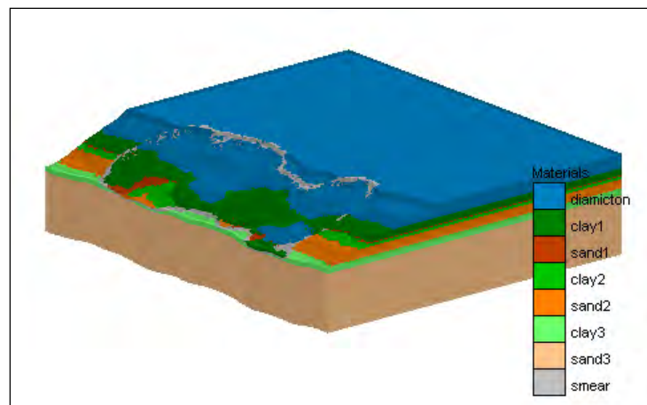
Figure 47. Finished computational mesh with material types assigned (Hansen et al. 2004).
