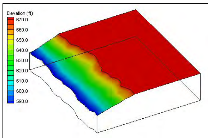
Figure 45. TIN describing the ground surface (Hansen et al. 2004).
