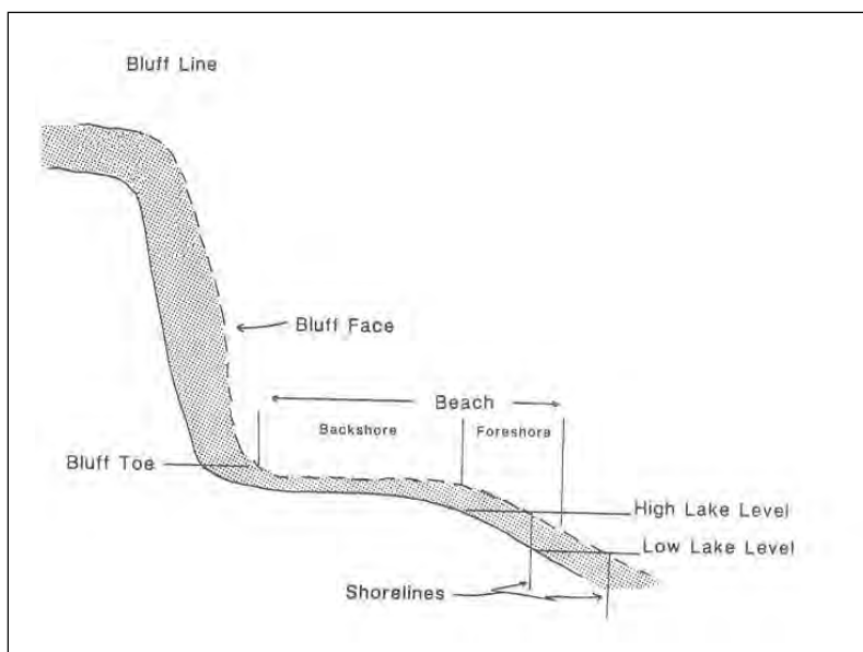
Figure 6. Lake bluff morphology for Allegan County (after Raphael et al. 1988).
