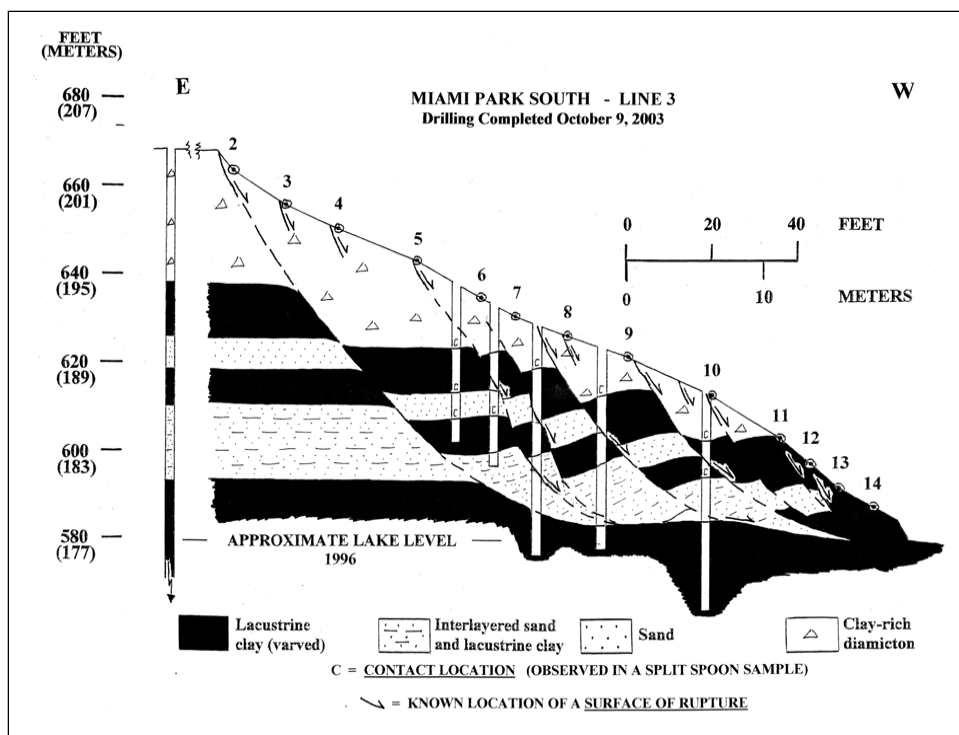
Figure 21 (continued). Part C, Survey Line 3 (by Chase).
