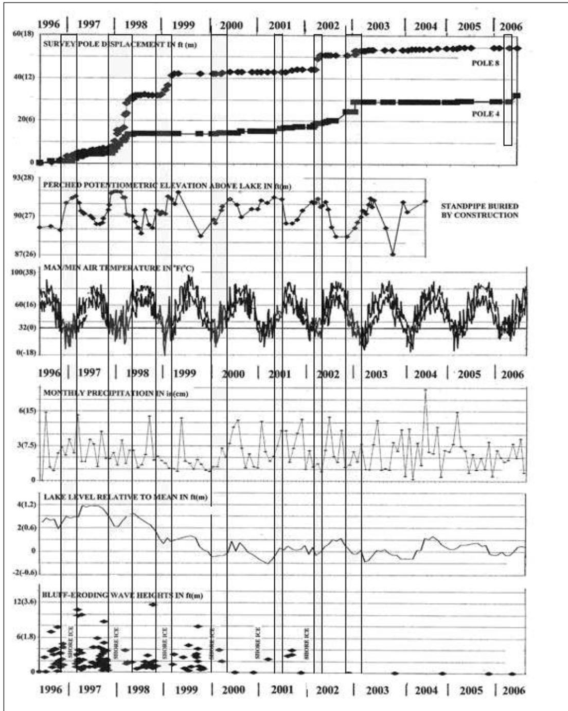
Figure 39. The pole (4 and 8, in dewatered section of MPS) and cable (Line 2) data, plus all temporal relations regarding groundwater, climate, precipitation, and wave action, compiled through September 2006 at MPS. Dewatering cycle, November 2004-May 2005, showed marked decrease in pole movement (after Chase et al. 2007b).
