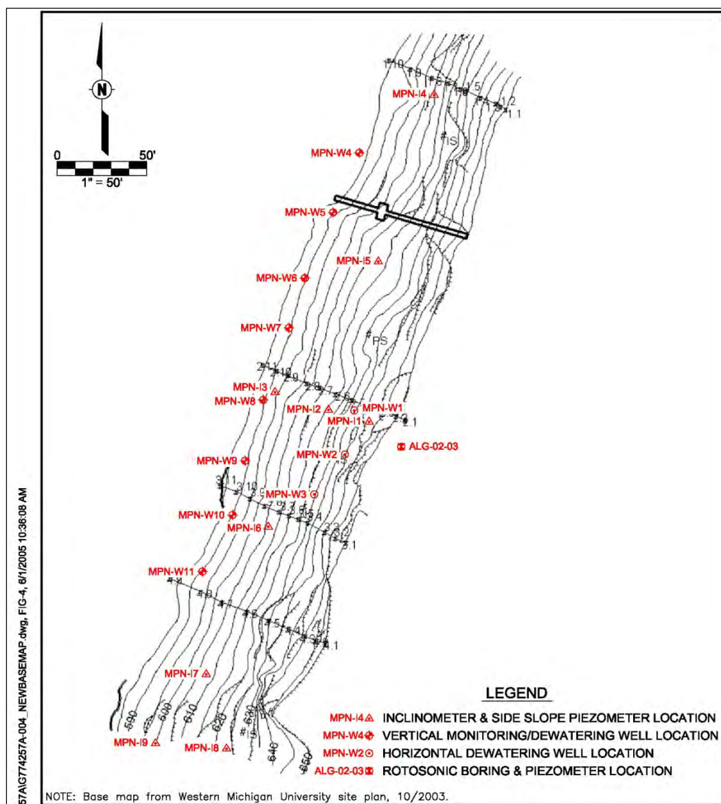
Figure 12. MPN site plan view showing locations of survey lines, instruments, and well locations. Perennial Seeps (PS) locations identified (after STS 2005, contour map by Ronald B. Chase).
