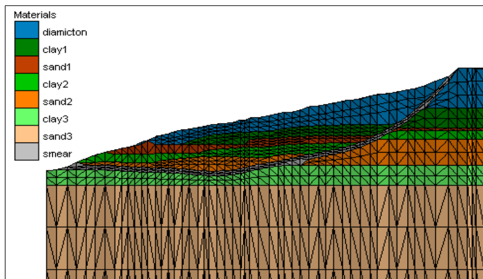
Figure 48. Typical cross section of finished computational mesh. The mesh has 124,786 nodes and 693,691 tetrahedral elements (Hansen et al. 2004).
