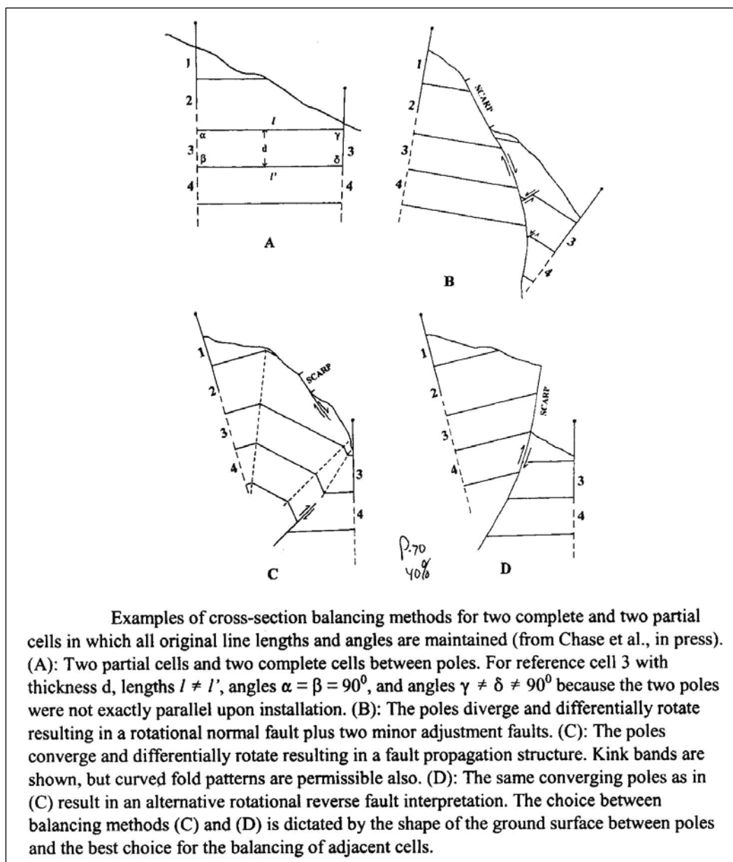
Figure 20. Description of the Balanced Cross Section Method (after Chase et al. 2001b).
