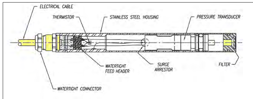
Figure 35. Piezometer schematic, downhole electronic pressure transducer with thermistor (after Roctest 2008).
