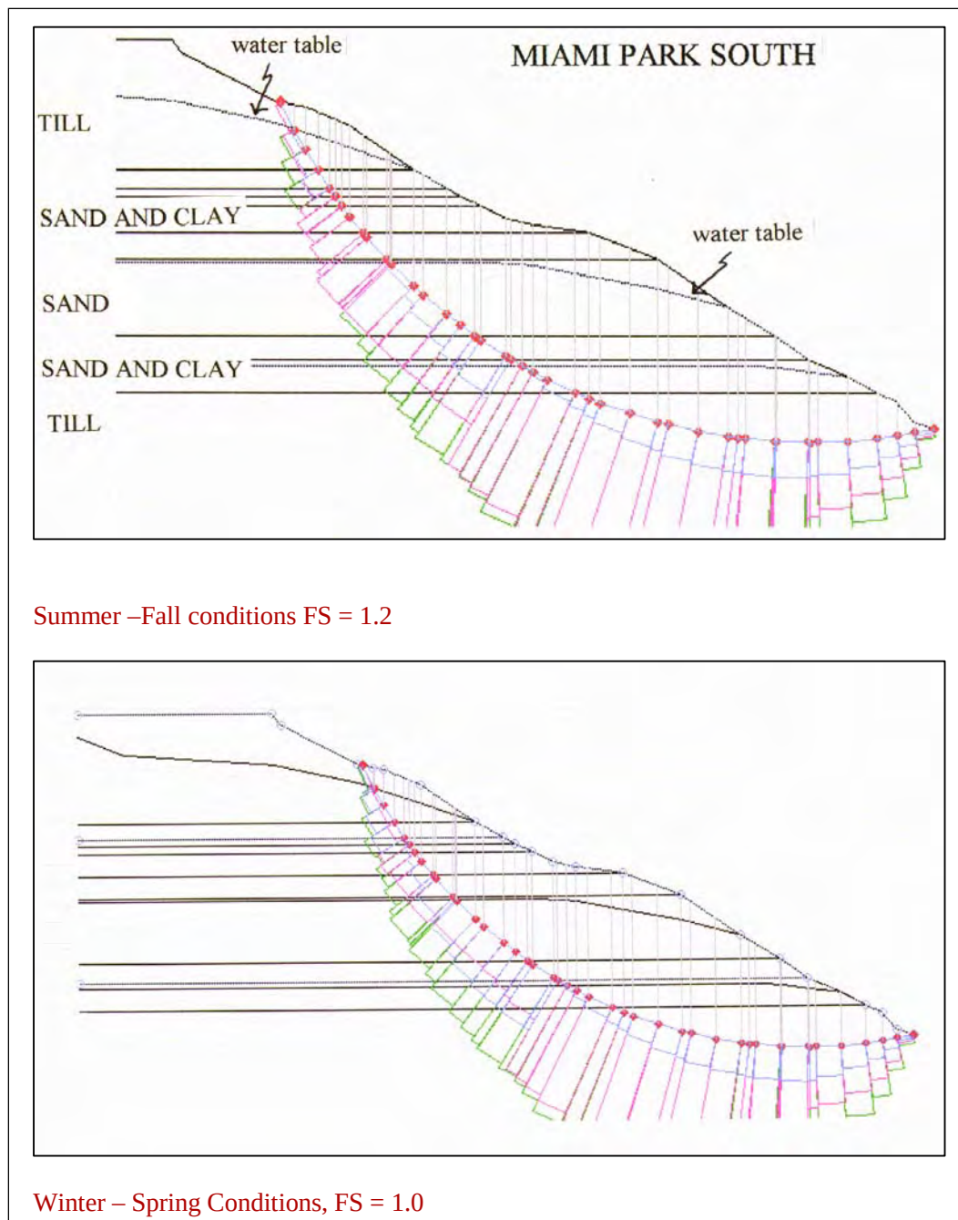
Figure 25. Graphic result of limit equilibrium analysis of Slip Surface 1 in Figure 26. Results of computer simulations (Spencer Method). Space between red dots width of slices. Force vectors at the base of each slice. Total stress = green, effective stress = red, and pore pressure = blue (after Chase et al. 2007b).
