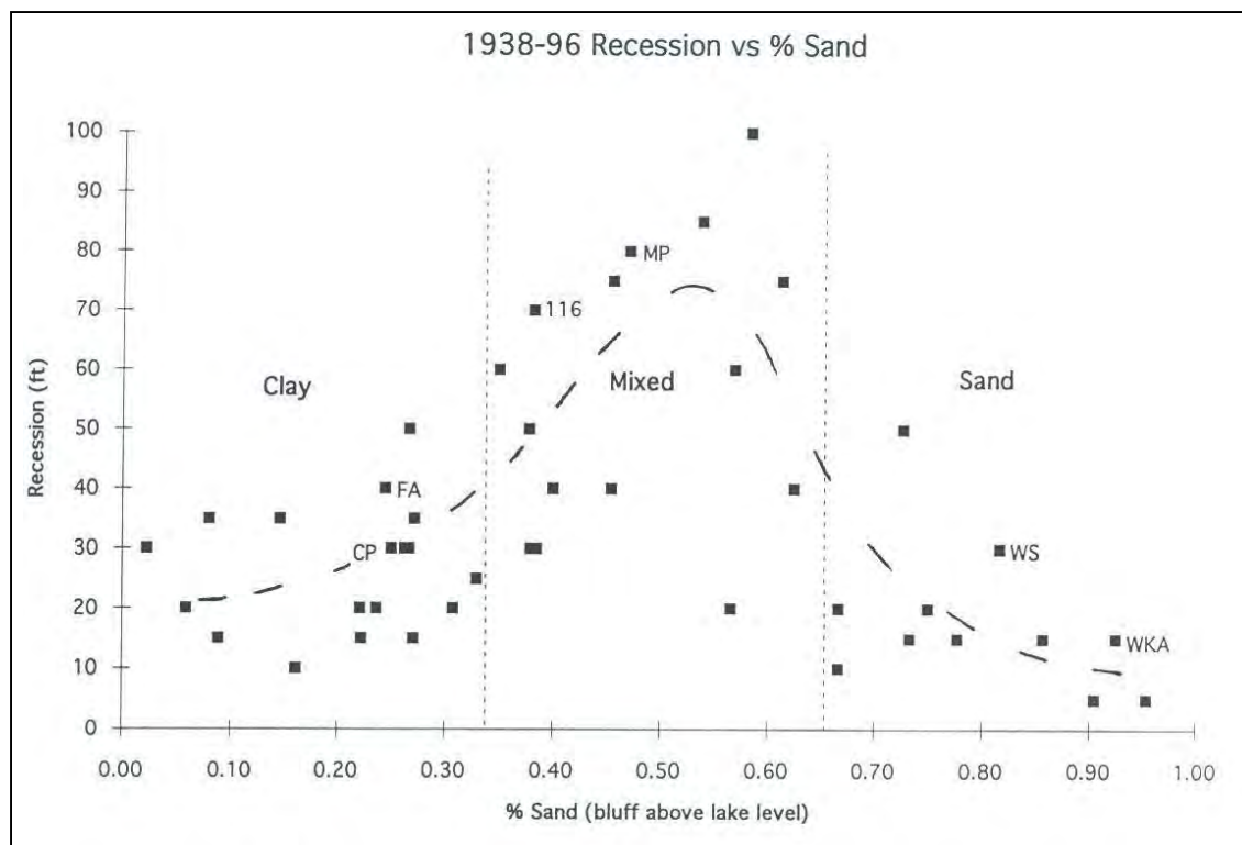
Figure 16. Recession rate versus bluff lithology (after Chase et al. 2007b)
