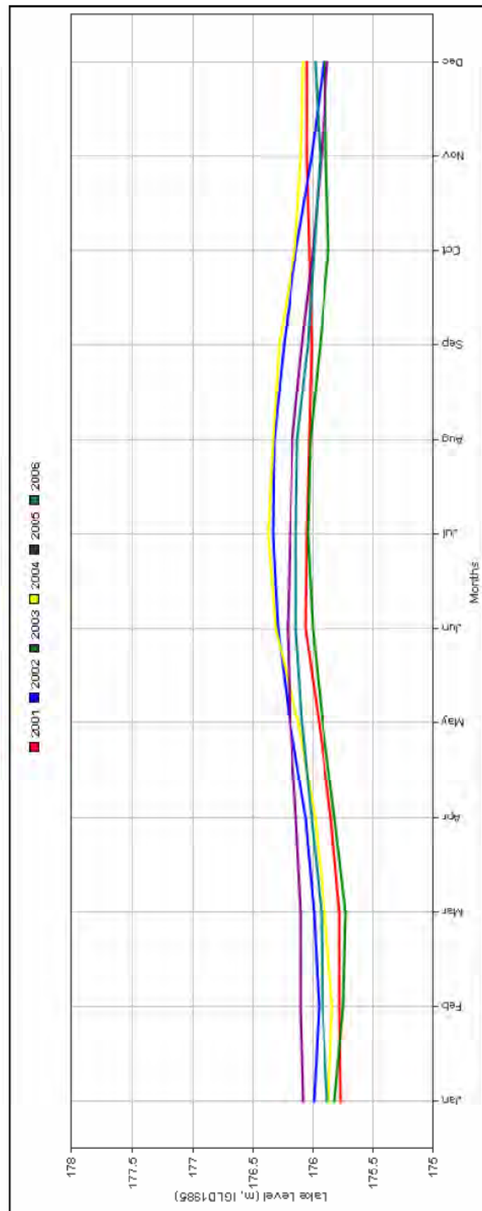
Figure 22. Part B, lake levels in meters, from 2001 to 2007 (USACE, Detroit District, 2008).
