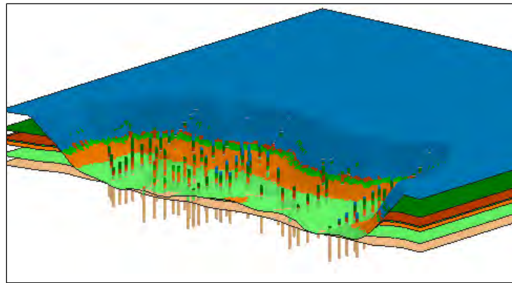
Figure 46. Figure showing borehole location and corresponding stratigraphic information applied to the groundwater model (Hansen et al. 2004).
