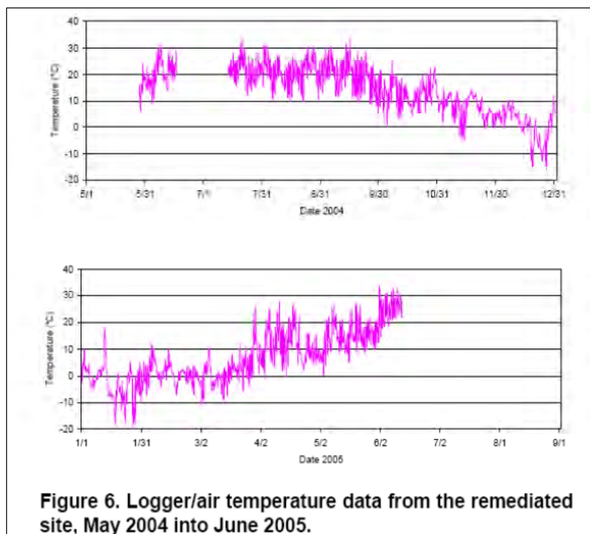
Figure 40. CRREL air temperature data, MPS, May 2004 to June 2005, recorded by data logger. This plot compares well to air temperature plotted by weather station at MPS. Data gap in June and July 2004 was because of an equipment setup error (Ferrick et al. 2005).
