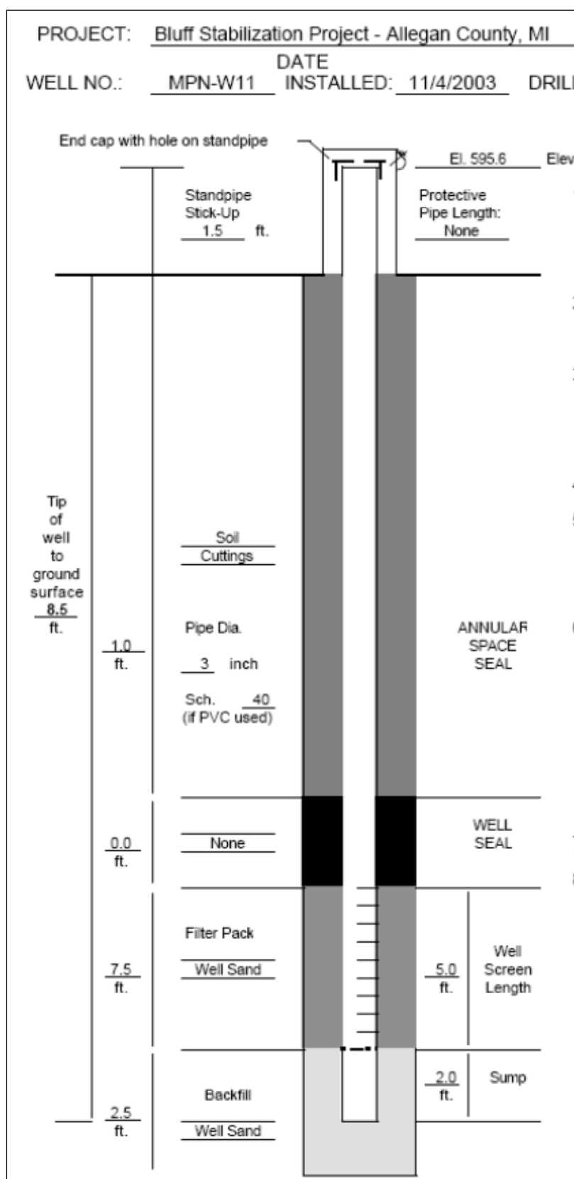
Figure 28. Field well installation diagram (after STS 2005).
