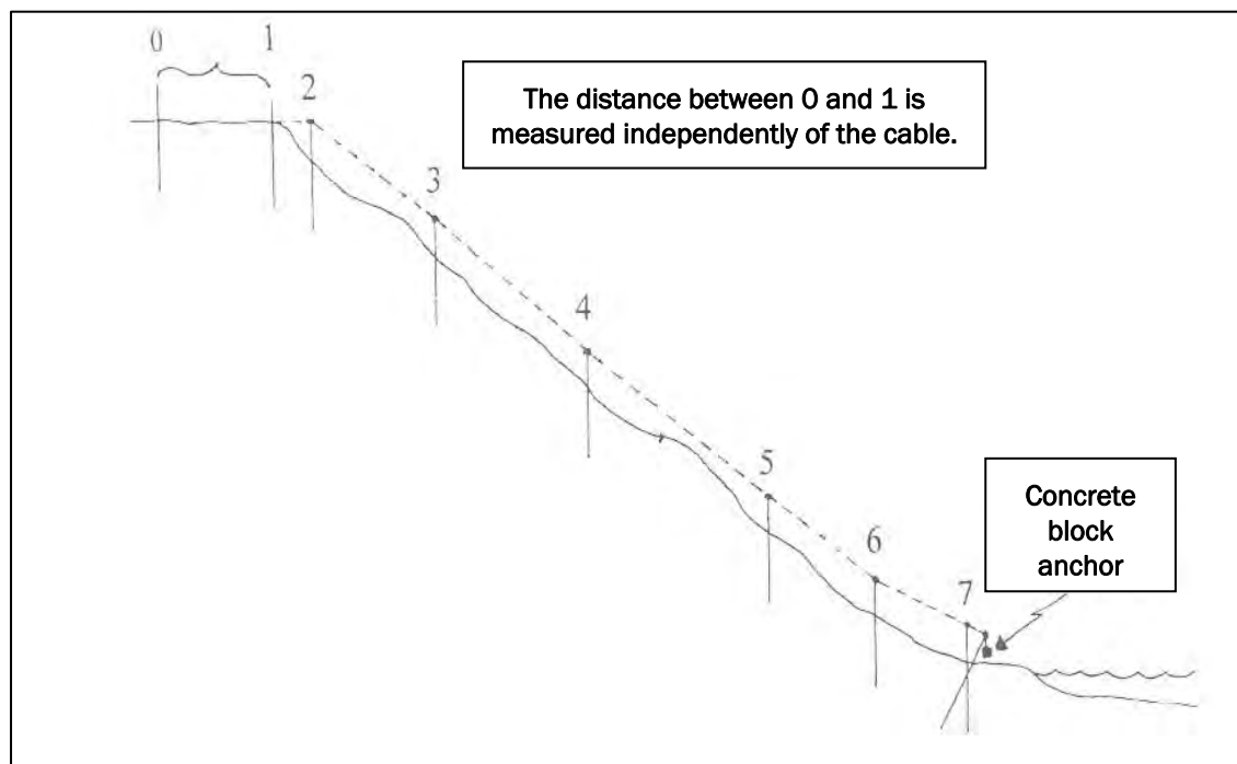
Figure 17. Example of pole-cable survey system. Poles should be anchored in clay layers (after Chase et al. 2001b).
