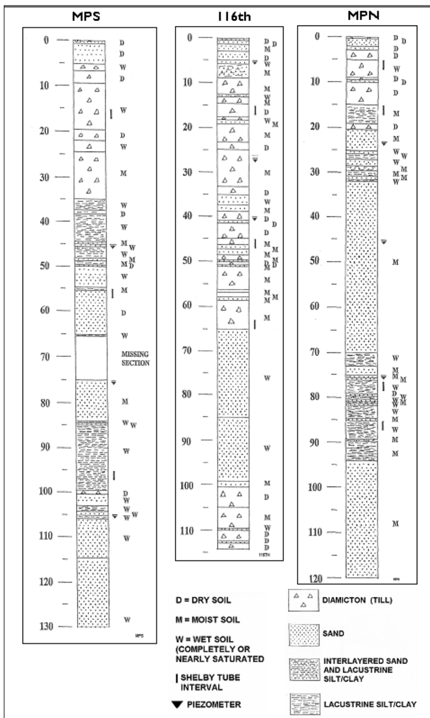
Figure 8. Geologic logs of roto sonic borings, from left, ALG-01 (MPS), ALG-02 (116th), and ALG-03 (MPN). Installed vibrating wire piezometers (VWPs) in each boring, 2004 (geologic interpretation by Ronald B. Chase).
