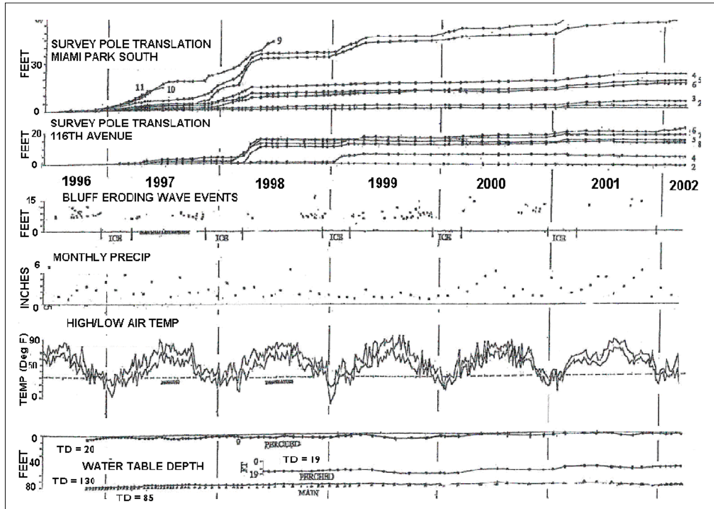
Figure 27. Plot showing annual trends in wave events, monthly precipitation, ambient air temperature, and water table depths below the bluff top and their correlations to slope movement at MPS and 116 th Avenue. Only those storm events with wave heights sufficient to reach the base of the bluff are plotted.
