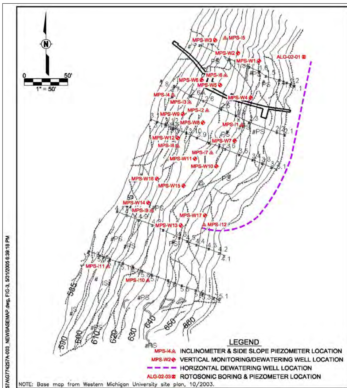
Figure 10. MPS site plan view showing locations of survey lines, monitoring instruments, and wells (after STS 2005; contour map by Ronald B. Chase).
