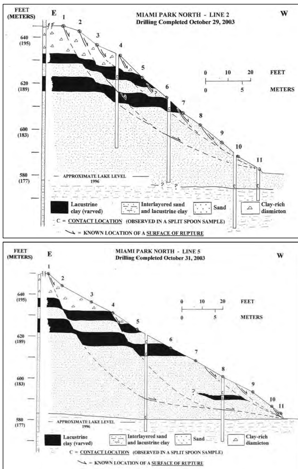
Figure 31. MPN, Line 2, top, and Line 3, bottom, cross sections, modified after drilling instrument and well borings. Note the large percentage of sand in the sections (cross sections interpreted by Ronald B. Chase). Error on bottom figure: Line 3, not 5.
