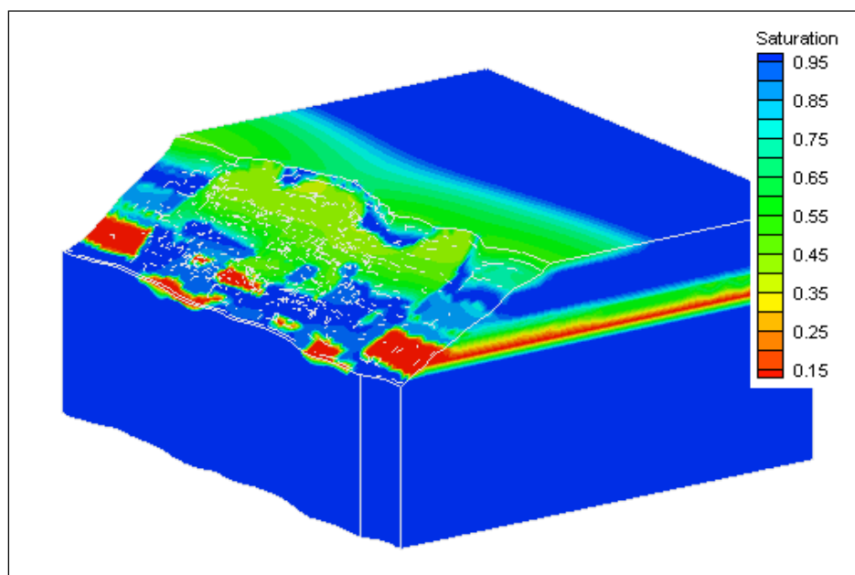
Figure 50. Model correctly locates flow from the bluff face above low permeable layers that contact higher permeable layers (sand) (Hansen et al. 2004).
