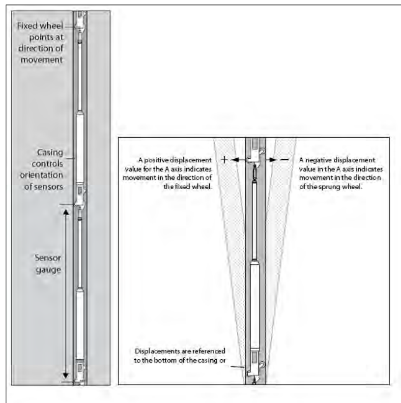
Figure 36. Schematic of downhole inclinometer, instrument for measuring deflection of borehole (deflection is measured in five separate locations within this borehole) (after Slope Indicator Manual 2008).
