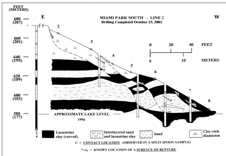
Figure 21 (continued). Part B, Survey Line 2 (by Chase).
