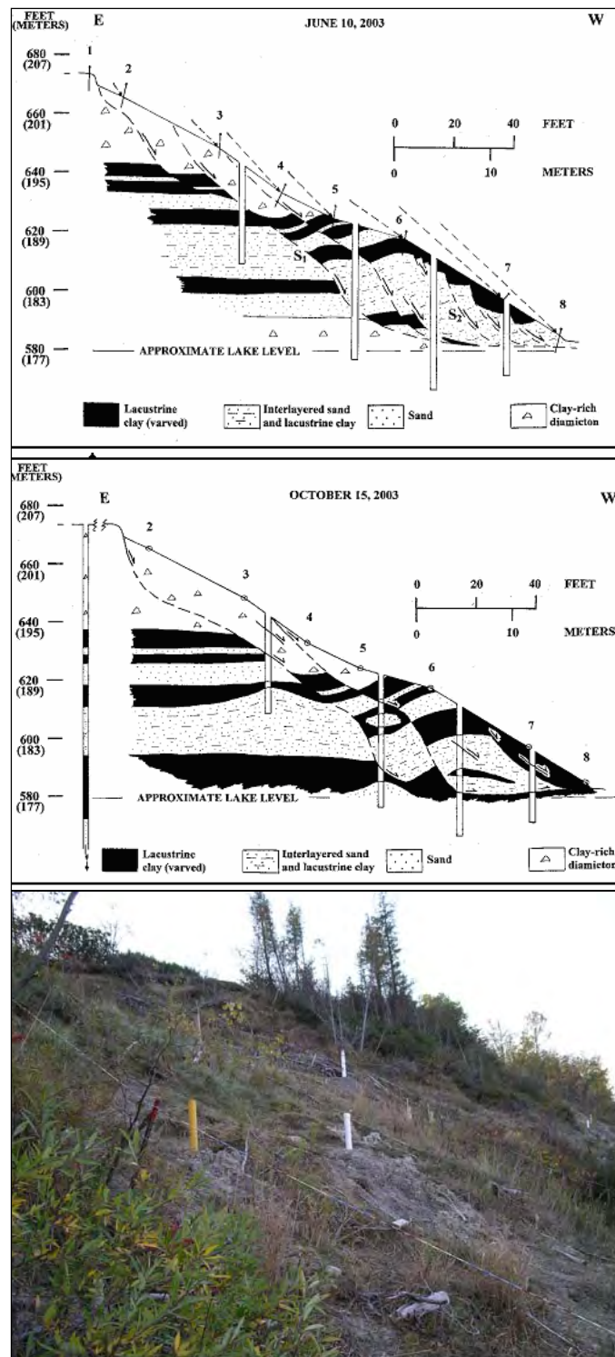
Figure 30. Stratigraphic contacts and slumping, from top, inferred-constructed in June 2003 using the Balanced Cross Section Method (after Chase et al. 2007a) and standpipe boring geology; modification of top cross section (by Ronald B. Chase) after drilling four instrumentation borings; and MPS wells and inclinometers, installed.
