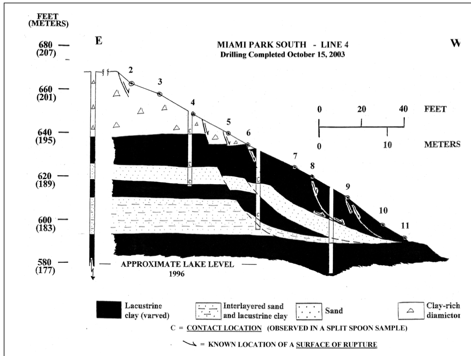
Figure 21 (continued). Part D, Survey Line 4 (by Chase).
