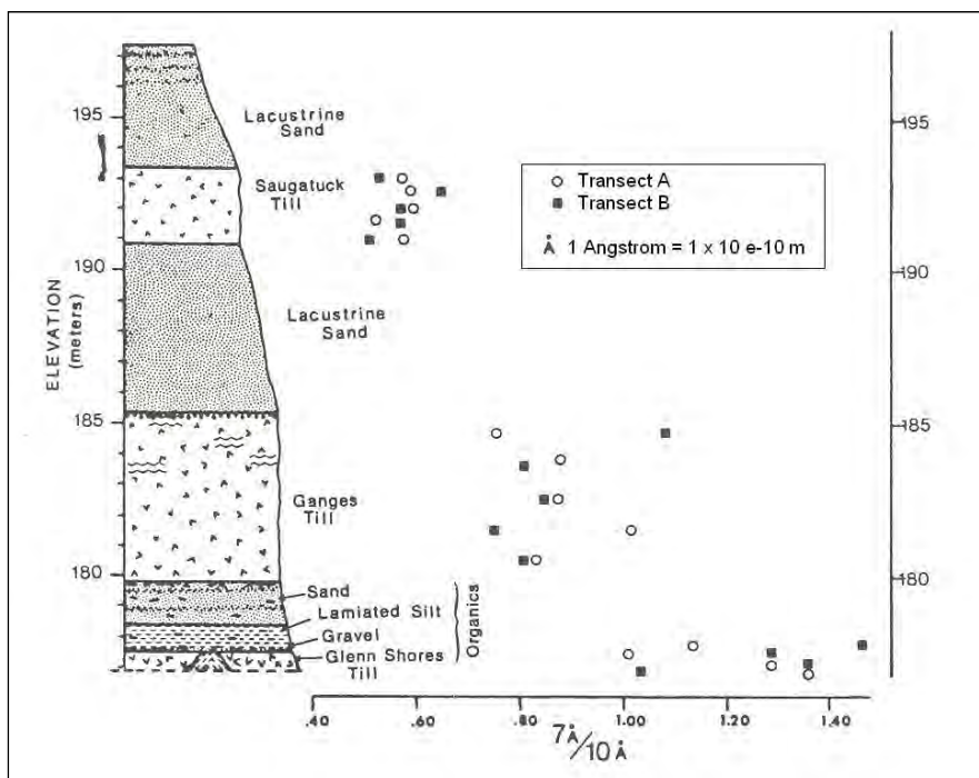
Figure 4. Regional stratigraphy (after Monaghan et al. 1986).
