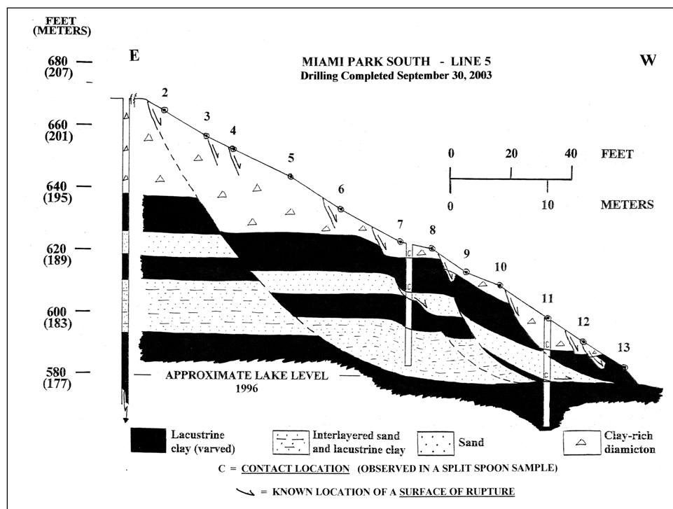
Figure 21 (concluded). Part E, Survey Line 5 (by Chase).
