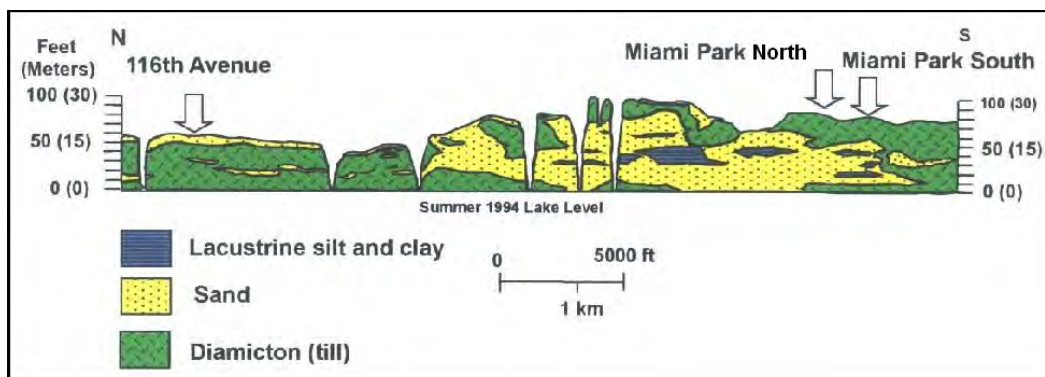
Figure 7. Six-mile profile showing detailed stratigraphy for the local area and between the 116th and MPS sites (after Chase et al. 2007b).
