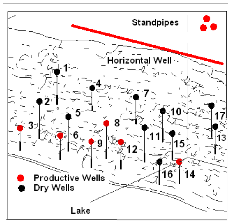
Figure 44. Extraction well locations. Red wells indicate productive pumping wells in May 2004. Black wells were dry in May 2004 (after Hansen et al. 2007). Note the upper-bluff wells are dry and lower-bluff wells are mostly wet (after Hansen et al. 2004).
