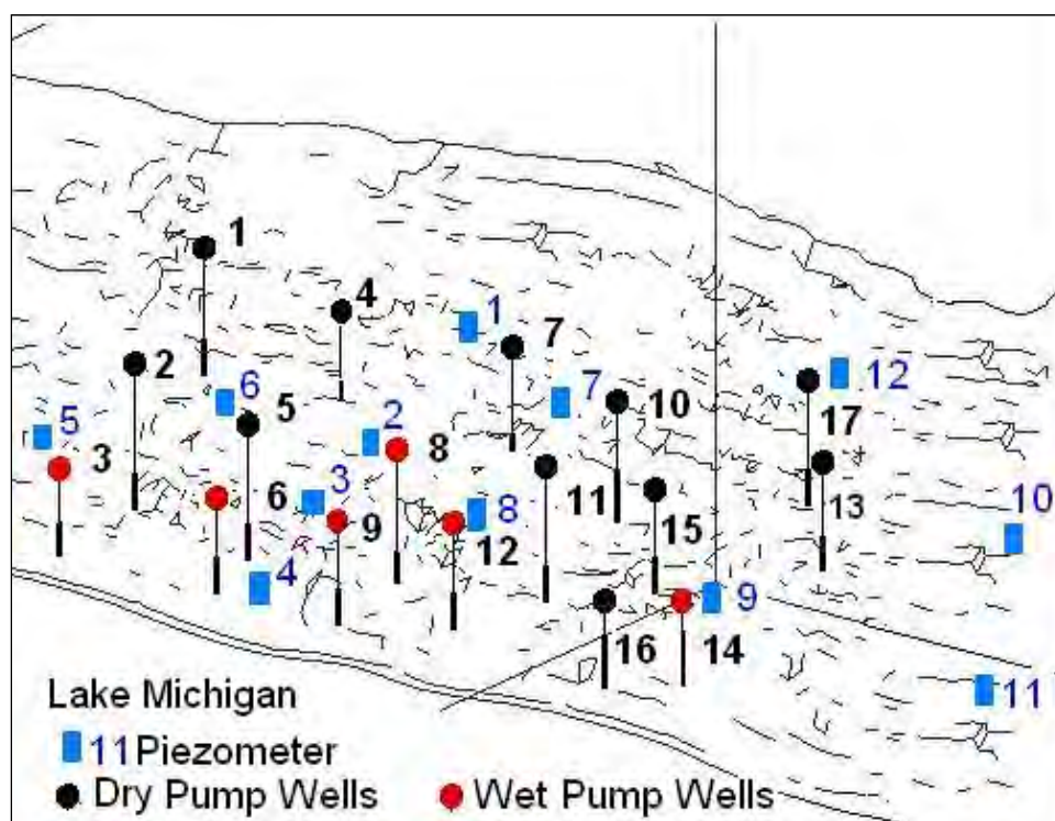
Figure 49. Piezometers and wells on bluff face (Hansen et al. 2007) combine the two figures above (Hansen et al. 2004).
