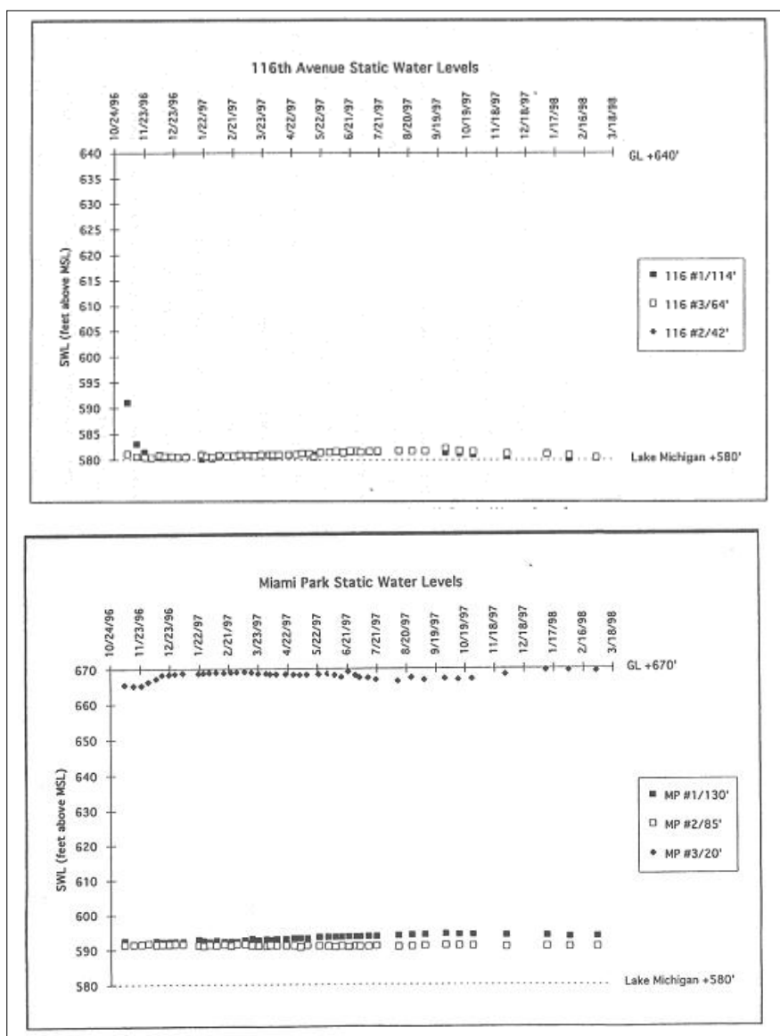
Figure 15. Piezometric readings (after Montgomery 1998).
