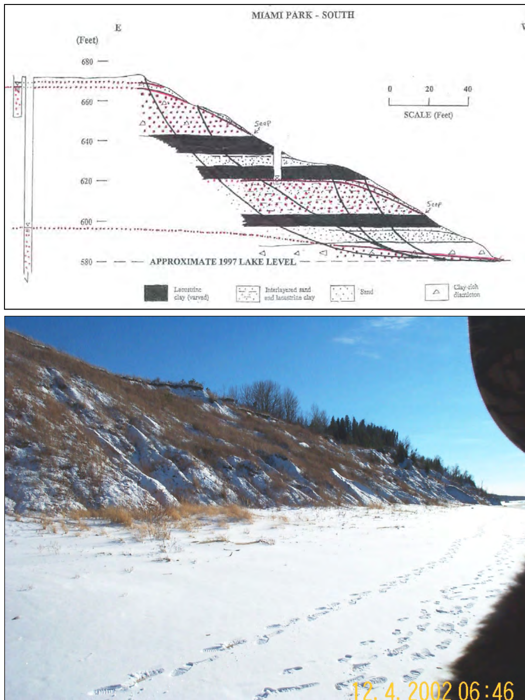
Figure 9. Model cross section, top, (by Ronald B. Chase) showing groundwater seeps and interpreted failure slip surfaces, with respect to bluff stratigraphy, bluff height, and above average 1997 lake level (Chase 2003, personal communication); bottom photo, MPS bluff in winter 2002.
