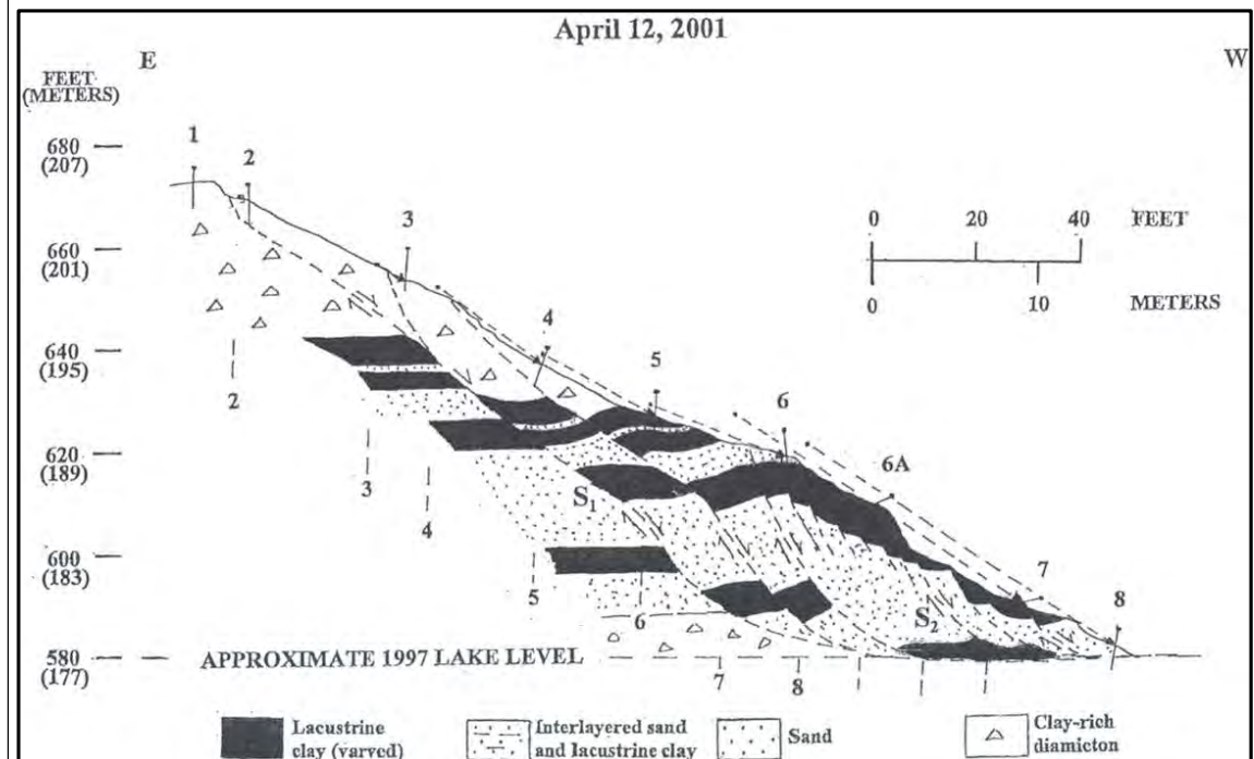
Figure 19. (a) Original position of poles at MPS (after Chase et al. 2001b) and (b) displacement of poles five years later. Cross-section b interpreted by Ronald B. Chase, using the Balanced Cross Section Method (Chase 2003, personal communication).
