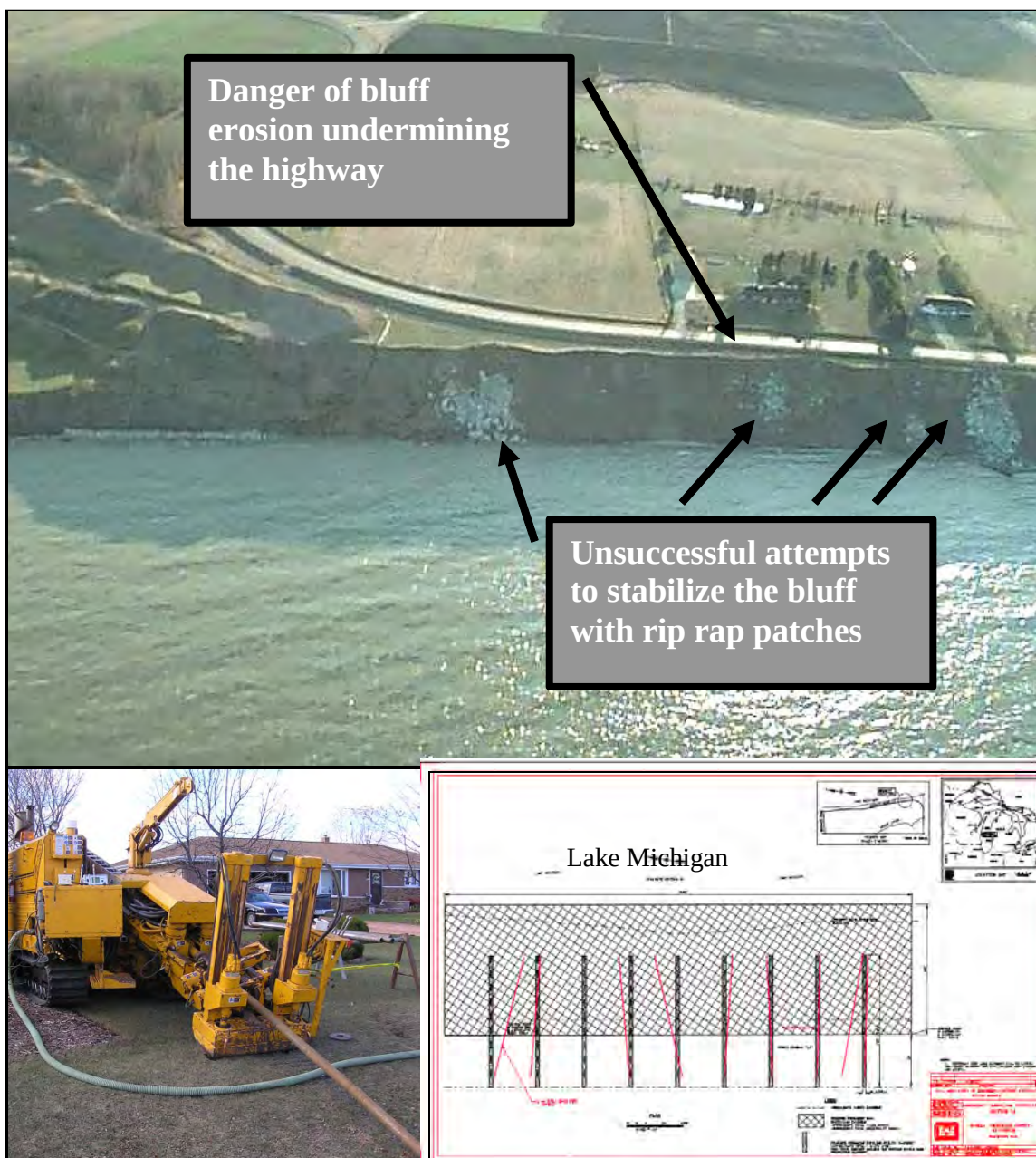
Figure 51. Mosel Bluff, clockwise from top, Lake Shore Road, Sheboygan County Wisconsin; directional drill rig atop Mosel Bluff and landside of Lake Shore Road; and as-built, plan view: nine directionally drilled drains from landside of Lake Shore Road to bluff toe (photos courtesy of Ross, USACE Detroit District; as-built courtesy of USACE, Detroit District).
