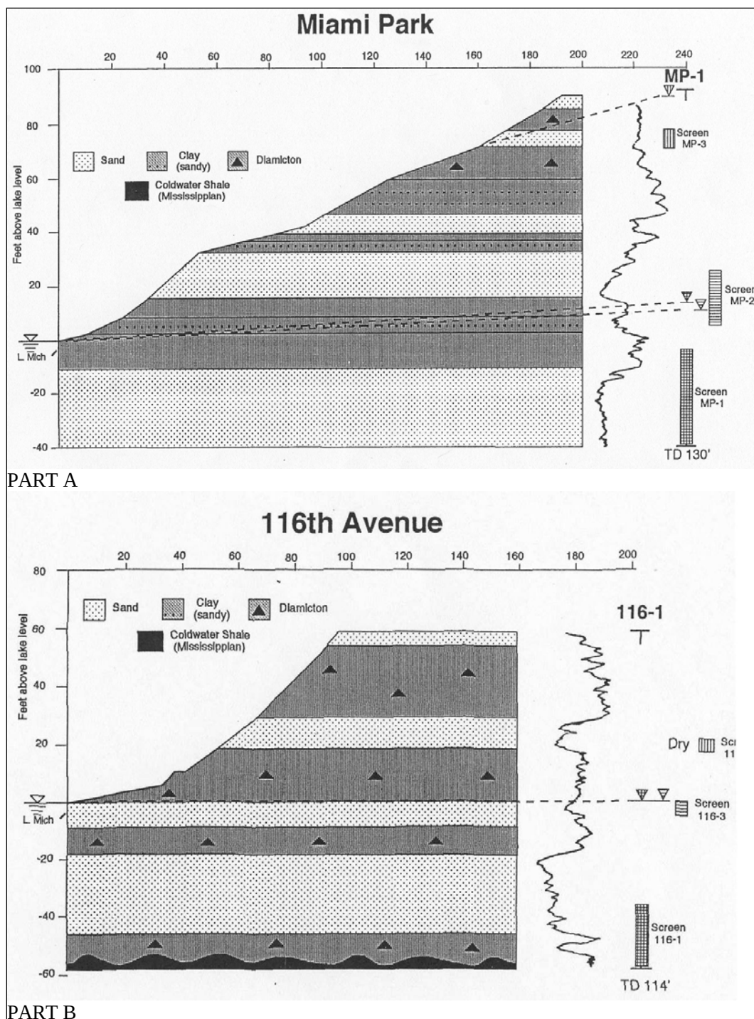
Figure 33. MPS and 116 th Avenue initial sections. Depths of standpipe piezometers and gamma ray log shown to the right of section. Water level data is from the Montgomery open standpipes between 1996 and September 2002. The rotonsonic VW piezometers (three per well), installed in September 2002, were added to the open standpipe data through December 2004. The bluff-face piezometers, activated in November 2004, and the rotonsonic ones have supplied the data since then (cross sections after Montgomery 1998).
