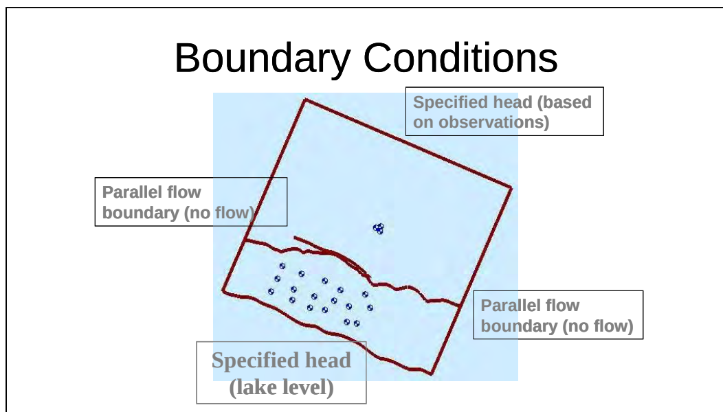
Figure 43. Illustration of numerical model's boundary conditions. Dimensions: length \approx 450 ft, width \approx 485 ft, and area \approx 200,000 ft 2 \approx 4.9 acres. Dewatering wells shown on the bluff face. Piezometer ALG-02-01 in center of the model. Three circles in the middle of the model represent open standpipes used for modified slug tests.
