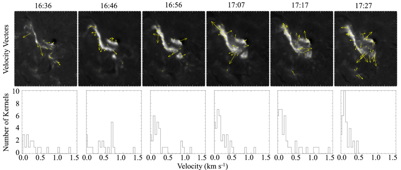
Figure 8. Time series of images with the apparent lateral velocity of each tracked flare kernel at that time step plotted over the H\alpha flare ribbons. A histogram of the number of flare kernels as a function of velocity corresponding to each time step is plotted underneath.
