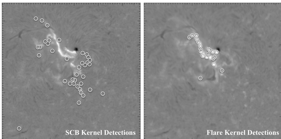
Figure 5. Example ISOON H\alpha images from the 2005 May 13 two-ribbon flare. The detection algorithm is applied to the image series to extract either ribbon brightening or compact brightening. The left image shows one time slice of individual SCBs identified external to the flare ribbon. The right image shows the same time slice with brightenings identified along the flare ribbon. Each detection is made up of a small matrix of pixels associated with the brightening called a kernel.
