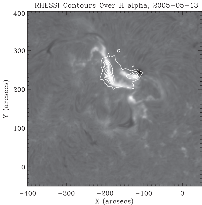
Figure 11. H\alpha image of the 2005 May 13 flare at peak intensity is shown with the reconstructed RHESSI 25–50 keV pass band integrated between 16:42 and 16:43 UT contoured on top at 10%, 30%, 50%, 70%, and 90% of the maximum intensity. The field of view of the RHESSI image [−220:−95, 180:305] is confined within the flaring region.
