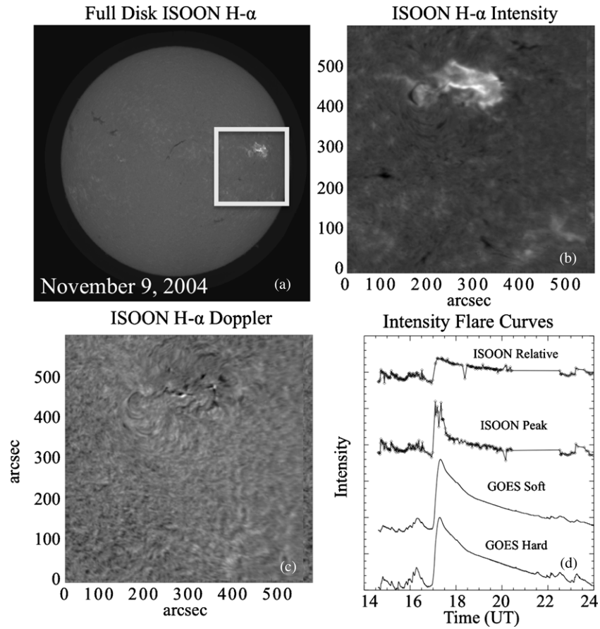
Figure 3. Two-ribbon flaring event from 2004 November 9. Panel (a) shows an example of a calibrated H \alpha ISOON image with the ROI highlighted. The ISOON images are 2048 \times 2048 pixels with each pixel having a 1''.1 resolution. Panel (b) is the ROI after preprocessing. This ROI covers 600 \times 600 pixels corresponding to 2.30 \times 10^{11} km ^2 on the solar surface. Panel (c) is a Doppler measure of the same ROI as part (b). The Doppler velocity image is created out of ISOON H \alpha off-band images described in Section 2 where the velocity ranges from -9.3 to 14.6 km s ^{-1} from black to white. Panel (d) shows intensity curves over the time period of interest: 14:37–23:58 UT as described in detail in the text.
