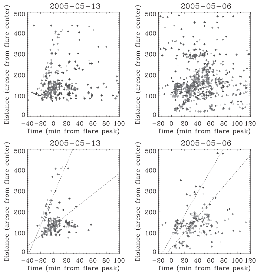
Figure 14. Derived statistics for all SCBs for the 2005 May 6 and 2005 May 13 events. All panels show the distance at which the SCB occurs vs. time from the H\alpha flare peak. The color of each plotted point is representative of its relative intensity; the lighter points are higher intensity detections. Bottom: the same plots as the top two panels except with a Doppler filter applied—each point had to have an SCB Type I Doppler shift associated with the line center brightening. The dashed lines are fit to the two visually distinct groups in each event.
