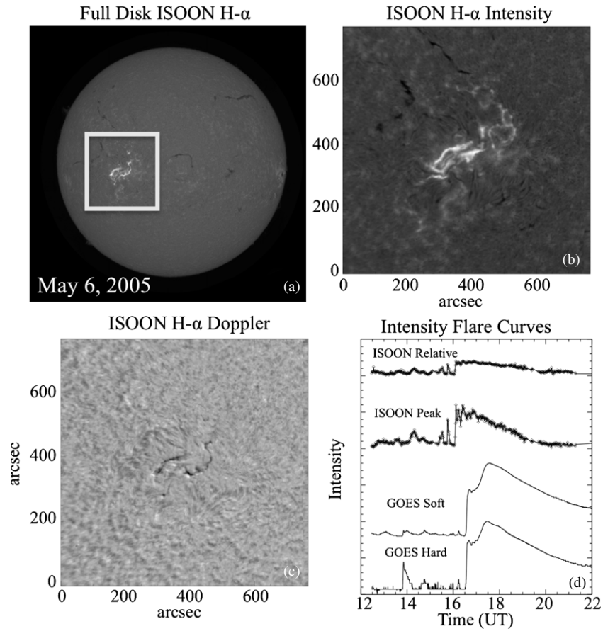
Figure 2. Two-ribbon flaring event from 2005 May 6. Panel (a) shows an example of a calibrated H \alpha ISOON image with the region of interest (ROI) highlighted. The ISOON images are 2048 \times 2048 pixels with each pixel having a 1''.1 resolution. Panel (b) is the ROI after preprocessing. This ROI covers 768 \times 768 pixels corresponding to 3.77 \times 10^{11} km ^2 on the solar surface. Panel (c) is a Doppler measure of the same ROI as part (b). The Doppler velocity image is created out of ISOON H \alpha off-band images described in Section 2 where the velocity ranges from -12.5 to 6.9 km s ^{-1} from black to white. Panel (d) shows intensity curves over the time period of interest: 12:28–22:47 UT as described in detail in the text.
