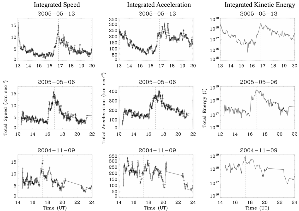
Figure 10. Integrated unsigned propagation speed, acceleration, and energy of flare kernels as a function of time for each of the three events studied. The vertical dashed line indicates the maximum flare intensity for the flaring event. The first column shows the integrated speed curves. The second column shows the acceleration of the flare ribbons. The third column shows the integrated kinetic energy, Equation (8), as a function of time for each of the three events studied. The 2004 flare had significant noise in the original data and a location on the limb contributing to the inconsistent measurements.
