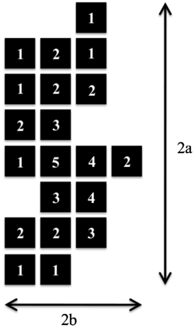
Figure 4. Diagram of a hypothetical kernel (either flare or SCB) used for classifications in this paper. Each pixel is labeled with a representative intensity [A_i] . The semi-major axis [a] and semi-minor axis [b] are shown. This kernel has the following properties: total intensity, m_0 = 43 , semi-major axis, a = 4 , semi-minor axis, b = 2 , eccentricity, e = 0.87 , centroid, (x, y) = (0.26, 0.18) , and radius of gyration, R_g = 1.9 . The maximum intensity, in this case 5, is defined as having pixel coordinates (0, 0) .
