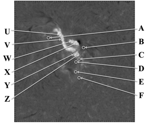
Figure 6. Image from the 2005 May 13 event. Letters A–F point to the locations several SCB kernels that are shown in more detail in Figure 7. Letters U–Z point to the locations of a sample of several flare kernels that are also shown in more detail in Figure 7. Note that since flare kernels move with the evolving flare ribbon, the locations of these kernels are only accurate for this image. In contrast, SCB kernels are stationary and remain in the same location in any image.
