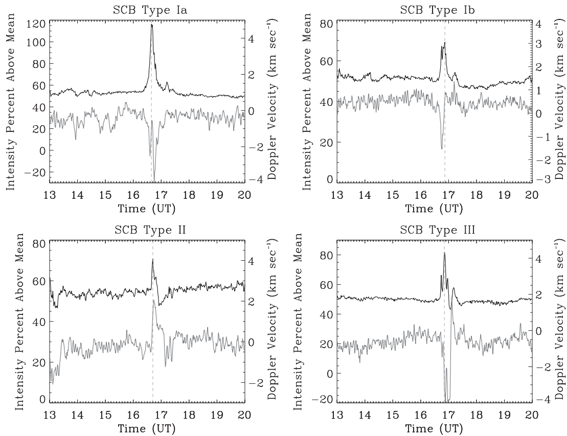
Figure 12. Line center intensity and Doppler velocity measurements for three different types of SCBs observed in both 2005 flares. The vertical dashed line marks the peak H\alpha intensity of the associated SCB. A negative Doppler velocity is away from the observer and into the Sun.
