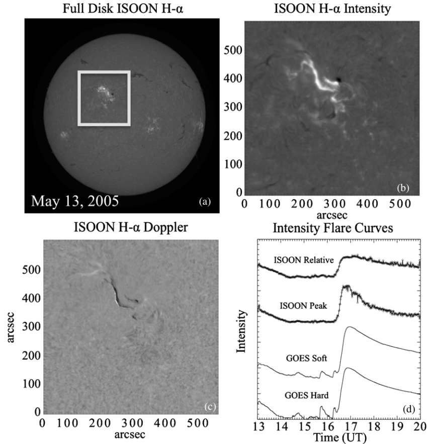
Figure 1. Two-ribbon flaring event from 2005 May 13. Panel (a) shows an example of a calibrated H\alpha ISOON image with the ROI highlighted. The ISOON images are 2048 \times 2048 pixels with each pixel having a 1''.1 resolution. Panel (b) is the ROI after preprocessing. This ROI covers 576 \times 576 pixels corresponding to 2.12 \times 10^{11} km 2 on the solar surface. Panel (c) is a Doppler measure of the same ROI as part (b). The Doppler velocity image is created out of ISOON H\alpha off-band images described in Section 2 where the velocity ranges from -26.6 to 21.5 km s -1 from black to white. Panel (d) shows intensity curves over the time period of interest: 13:00–20:02 UT as described in detail in the text.
