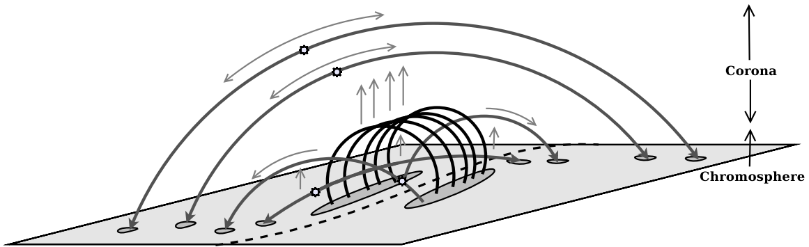
Figure 16. Schematic model of the physical cause of SCBs. A dashed line marks the neutral line in this model. The central loops represent the emerging two-ribbon flare arcade. The arches represent field lines connecting outside of the flare ribbons. The arrows on top of both the loops and arches show the direction trapped plasma flows as the flare begins to erupt and the stars suggest the location where the plasma is disrupted. Once perturbed, the trapped plasma streams down the loop lines and impacts the chromosphere causing the H\alpha intensity brightening. The different orientations of off-flare loops account for the different propagation speeds of SCBs observed.
