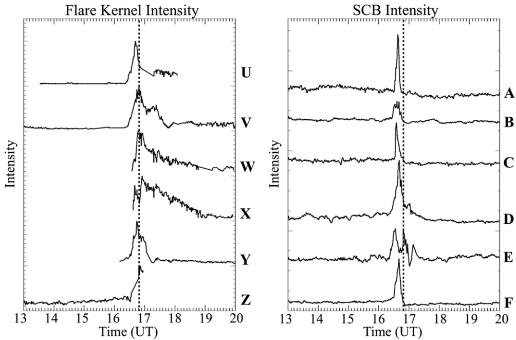
Figure 7. H\alpha normalized intensity curves for each of the kernels indicated in Figure 6 by the associated letters. On the left, the tracked flare kernels are shown. The normalized intensity curves for the SCB kernels, shown on the right, are stationary and therefore tracked throughout the flaring window. In both panels, the vertical dashed line indicates the time at which the flare intensity peaks (16:49 UT) derived from integrating all flare kernel intensities at each time step.
