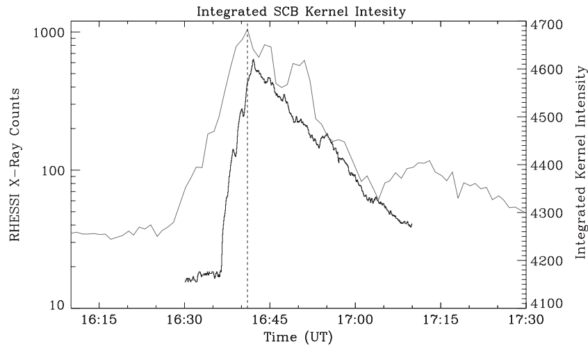
Figure 15. Plot showing the RHESSI non-thermal 25–50 keV intensity in black and the H\alpha SCB integrated intensity curve in gray for the 2005 May 13 flare. The vertical dashed line indicates the peak of the integrated SCB curve.
