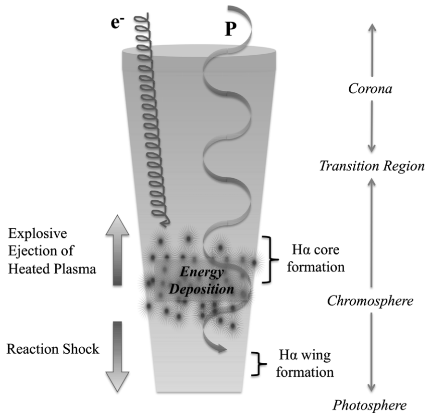
Figure 17. Diagram of the physical dynamics occurring in a single SCB. Electrons and protons accelerated by magnetic reconnection further up in the corona come streaming down the flare loop. Since the mean free path of electrons is significantly less, the electrons deposit energy into the upper chromosphere. Unable to radiate the energy as heat, the chromosphere explosively responds by sending material back up the flux tube (chromospheric evaporation) and a reaction shock propagates toward the photosphere. This reaction shock explains the velocities observed in Type I SCBs.
