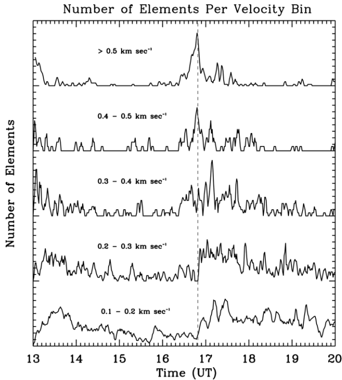
Figure 9. Number of elements in each apparent lateral velocity bin plotted as a function of time. The vertical dashed line marks the time of the peak flare intensity. The velocity bins are 0.1 \text{ km s}^{-1} in width. The smallest bin, 0-0.1 \text{ km s}^{-1} , is excluded because of a base level of noise inherent in the detection routine.
