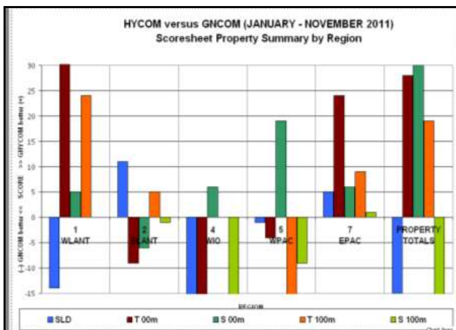
Figure 2.1. Bar graph of HYCOM scores for each property evaluated, by region, from Table 2.1. Positive scores (above the zero line) indicate a net "win" for HYCOM. All regions are summed by property to the right.
