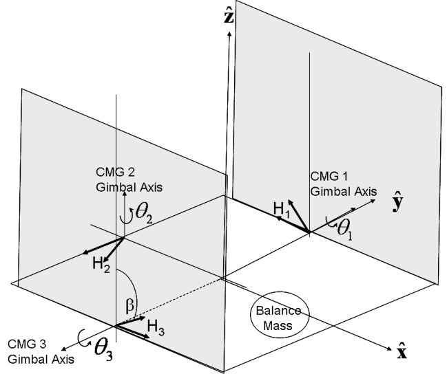
Fig. 9 \{\beta_1, \beta_2, \beta_3\} = \{90, 0, 90 deg \} mixed skew angle momentum cutting planes depicted for a 3/4 CMG skewed array.
