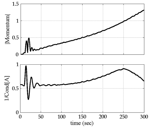
Fig. 12 Experiment: +5^\circ yaw in 4 s, -5^\circ yaw in 4 s, and then regulate for 5 min. Skew angles equal 90^\circ .
