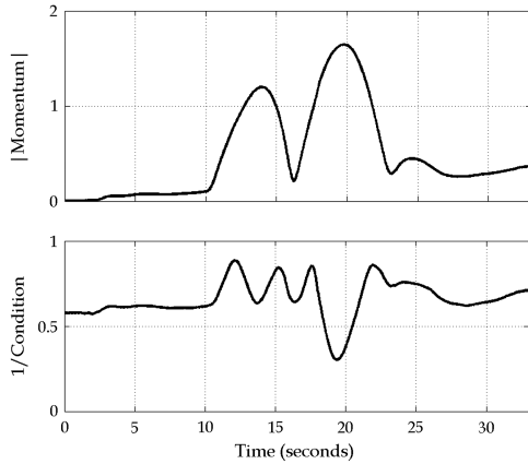
Fig. 15 Experimental results: +13 deg yaw in 4 s, and -13 deg yaw in 4 s performed in \{\beta_1, \beta_2, \beta_3\} = \{90, 0, 90 \text{ deg}\} mixed skew angle configuration (with maneuver momentum and inverse condition of [A] ).
