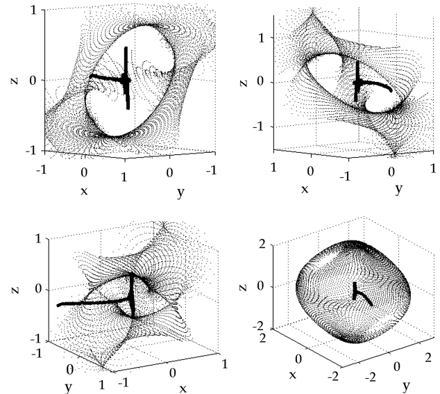
Fig. 13 Fictional experiment: Fig. 11 placed in context of 54.73^\circ momentum envelope.
