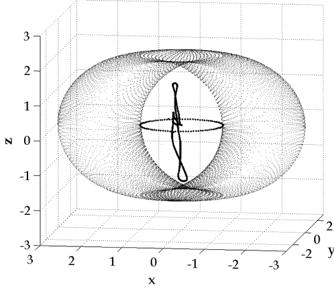
Fig. 14 Experimental results: +13 deg yaw in 4 s, and -13 deg yaw in 4 s performed in \{\beta_1, \beta_2, \beta_3\} = \{90, 0, 90 \text{ deg}\} mixed skew angle configuration. the momentum trajectory is placed in the context of theoretical singular hypersurface.
