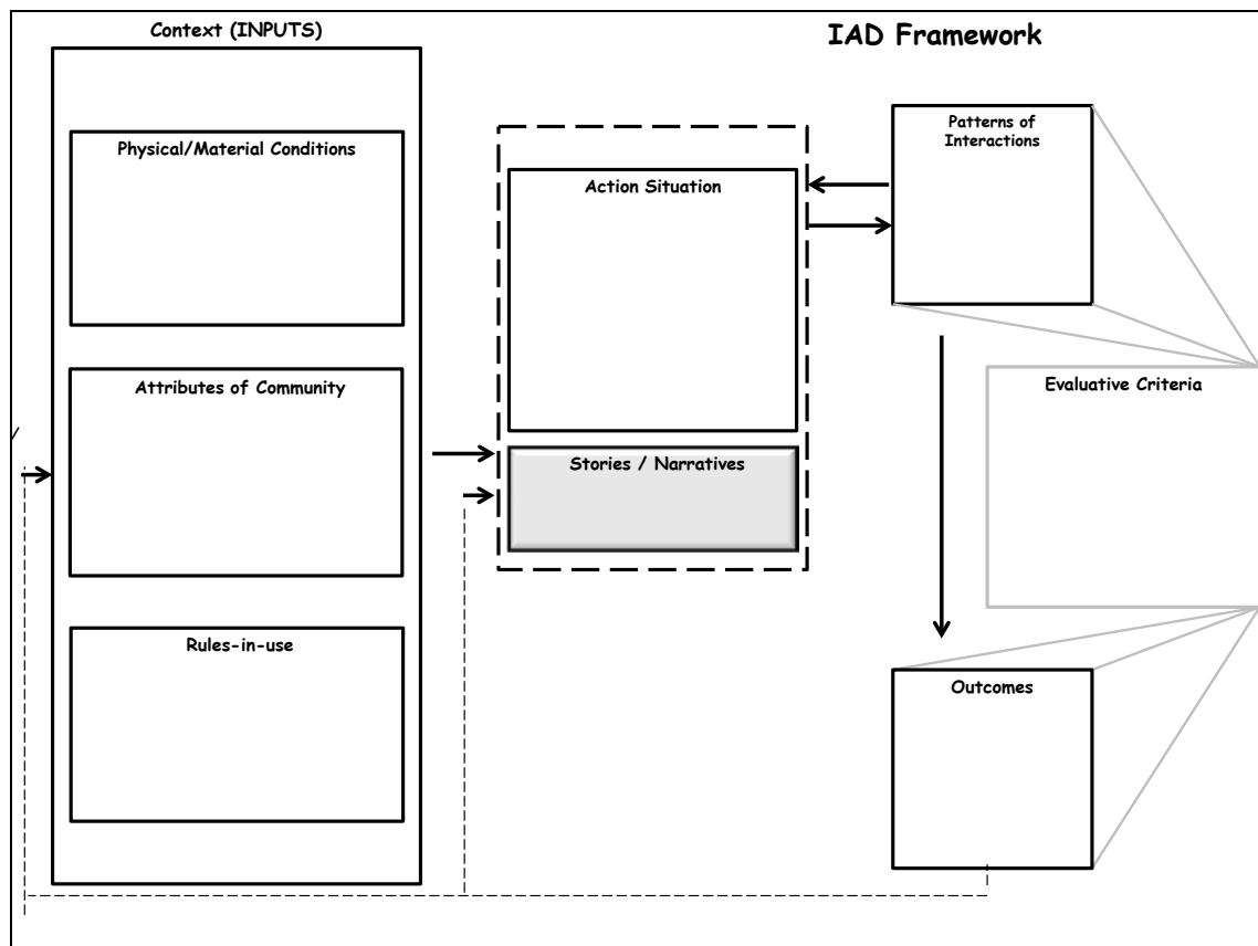
Figure 1. IAD Framework
