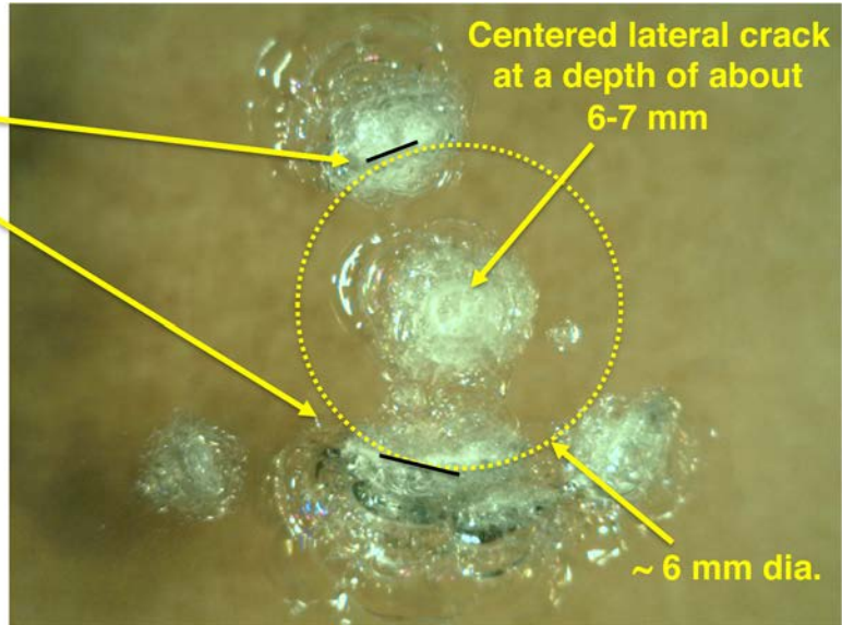
Figure 5.13. Example of multiple failure initiation locations on laser shock impacted Starphire soda lime silicate glass.
