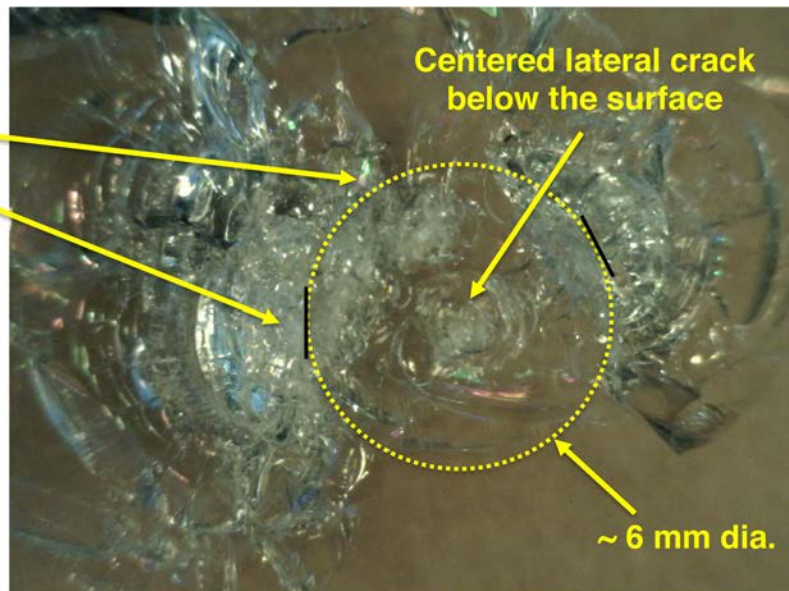
Figure 5.14. Example of multiple failure initiation locations on laser shock impacted BOROFLOAT borosilicate glass.
