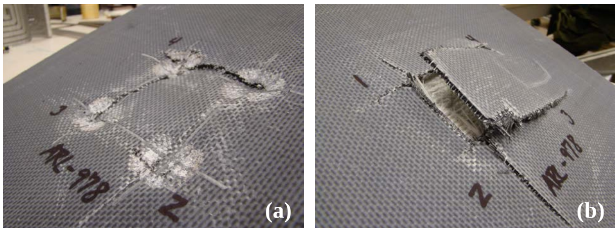
Figure 17. Front face (a) and back face (b) impact damage for Hybrid no. 3 (baseline).
