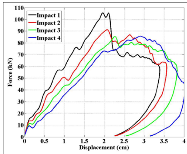
Figure 5. Force vs. displacement for Hybrid no. 3 (baseline).
