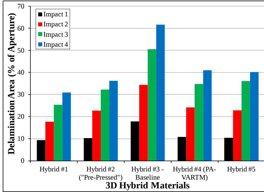
Figure 14. Delamination areas as a percentage of impact table aperture for each material.
