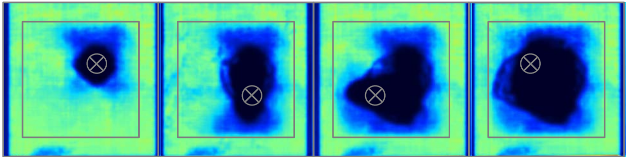
Figure 13. C-scan image showing progression of delamination in Hybrid no. 5.
