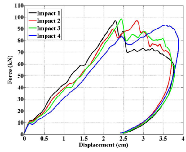
Figure 6. Force vs. displacement for Hybrid no. 4 (PA-VARTM).
