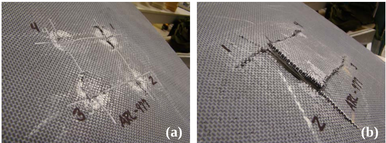
Figure 16. Front face (a) and back face (b) impact damage for Hybrid no. 2 ("pre-pressed").
