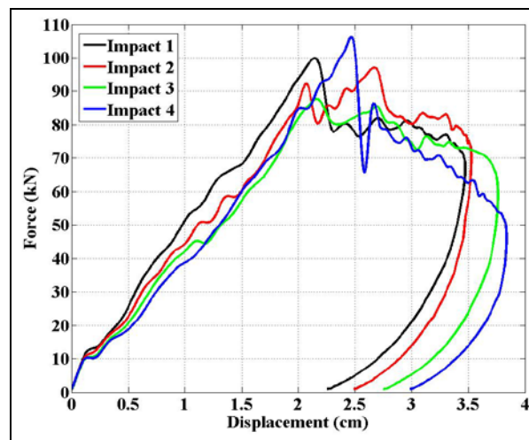
Figure 3. Force vs. displacement for Hybrid no. 1.
