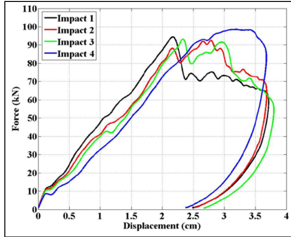
Figure 4. Force vs. displacement for Hybrid no. 2 ("pre-pressed").
