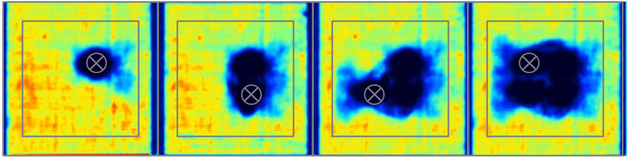
Figure 9. C-scan image showing progression of delamination in Hybrid no. 1.
