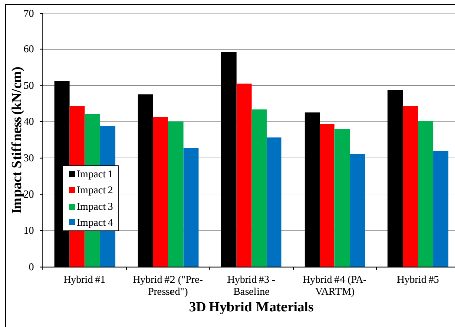
Figure 20. Initial impact stiffness for all hybrid materials.
