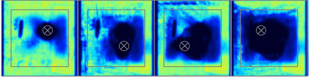
Figure 12. C-scan image showing progression of delamination in Hybrid no. 4 (PA-VARTM).
