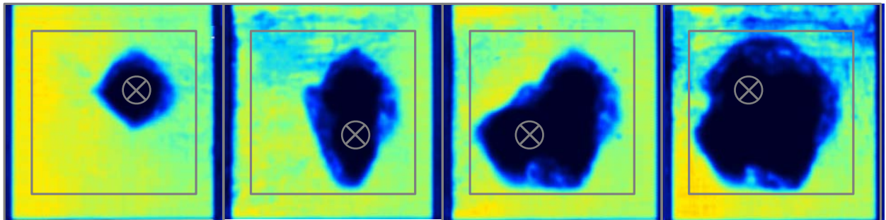
Figure 11. C-scan image showing progression of delamination in Hybrid no. 3 (baseline).
