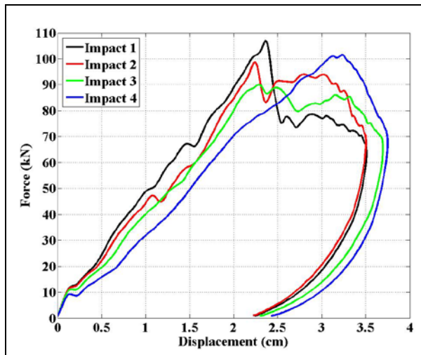
Figure 7. Force vs. displacement for Hybrid no. 5.
