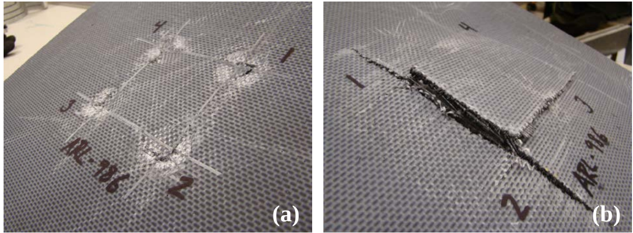
Figure 19. Front face (a) and back face (b) impact damage for Hybrid no. 5.
