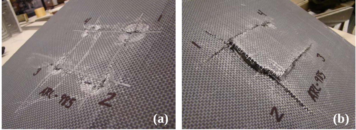
Figure 18. Front face (a) and back face (b) impact damage for Hybrid no. 4 (PA-VARTM).
