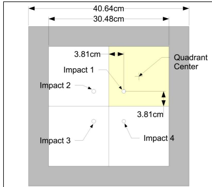
Figure 2. Illustration of the sample and impact location.
