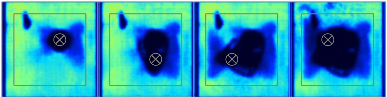
Figure 10. C-scan image showing progression of delamination in Hybrid no. 2 (“pre-pressed”).
