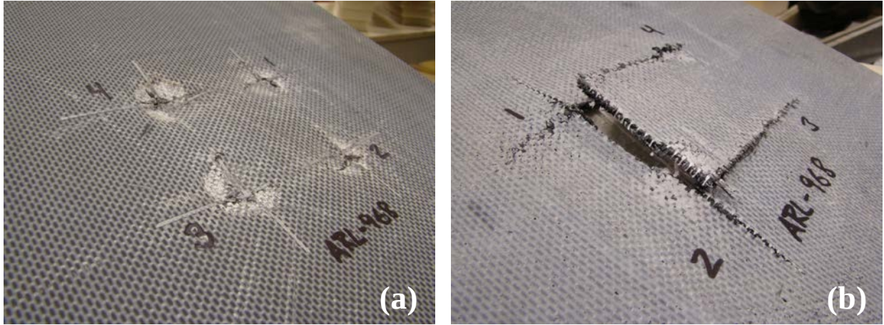
Figure 15. Front face (a) and back face (b) impact damage for Hybrid no. 1.
