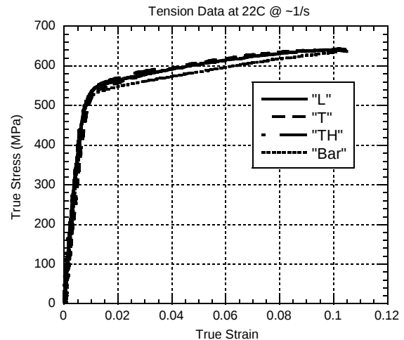
Figure 2. Tension data from 3/8" diameter bar stock and three directions from 1" thick plate.
