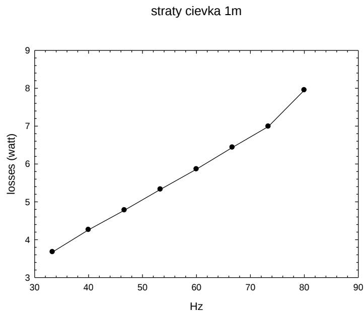
Fig. 9. Coil losses using the calibration curve in Fig.8.
