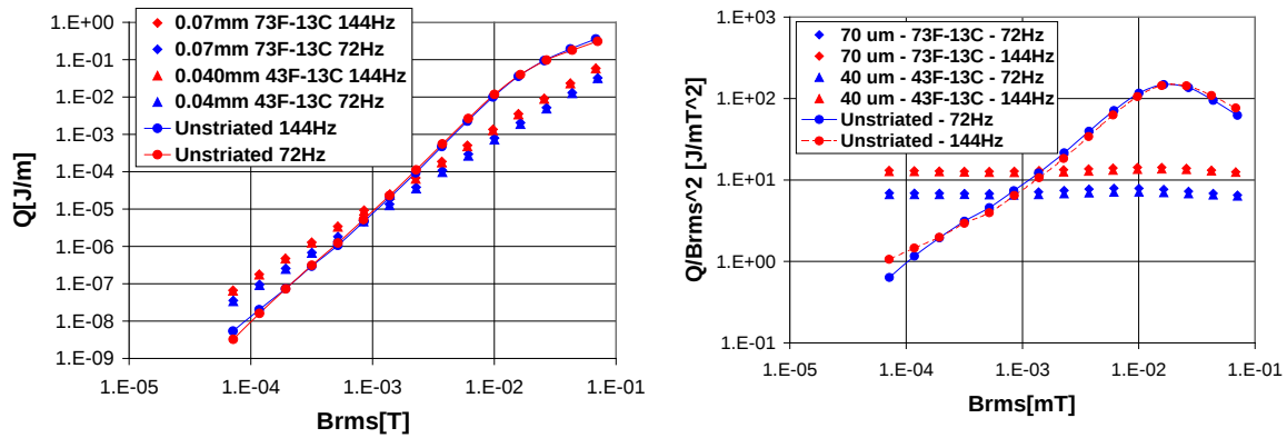
Figure 8. Ac magnetization loss of samples from set III in Q and \Gamma representation.
