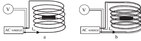
Figure 1. Set-up magnetization loss determination in the superconducting sample (black rectangle) based on the measurement of power supplied to the AC field magnet. (a) Measurement of total AC power delivered by the AC power supply; (b) modification to neglect the resistive loss in the AC field magnet.
