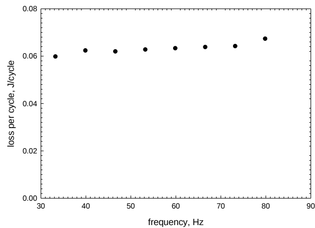
Fig.5. Losses per cycle as a function of frequency, determined using data from Fig. 4.
