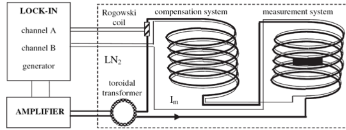
Figure 2. Measurement scheme allowing us to determine the AC loss according to the proposed method.
