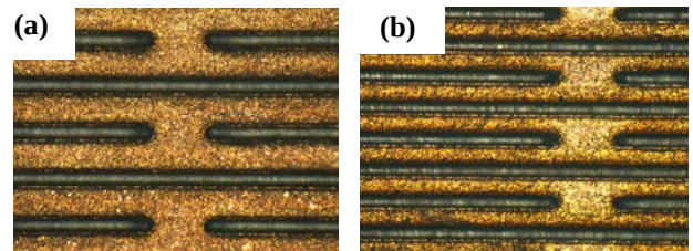
Figure 1(a,b) Striated samples with the laser cut grooves (shown at 10x magnification). The width of the individual stripes is 70 \mu\text{m} in Fig. 1(a) and 40 \mu\text{m} in Fig. 1 (b). Superconducting bridges facilitating current transfer between the individual stripes were left in some samples.
