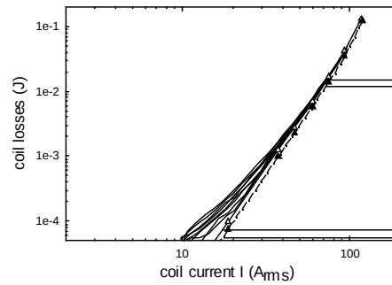
Fig. 8. Coil losses measured at frequencies from 22.5 to 135 Hz. Calculated losses: \pi - non-uniform current density, p - uniform current density
