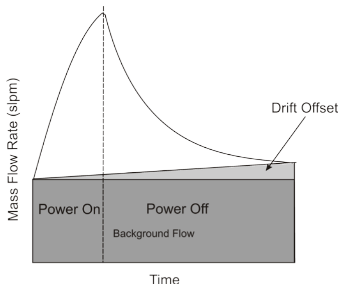
We have used a measurement protocol illustrated in Fig. 2. The current through the coil that generates losses was turned on for about three minutes. Over this period of time the outflow of gas increases. When the current is turned off, the mass flow gradually decreases reaching the background level. Thus, knowing the total amount of evaporated nitrogen above the background level, and correcting for background flow drift, we can calculate the total excess of energy deposited into the pool of \text{LN}_2 by the coil. Dividing this energy by the time the current was running, we obtain the power loss. Our estimates based on heat capacity of the coil indicate that the maximum temperature rise inside the coil was of the order of 1 K or less.
