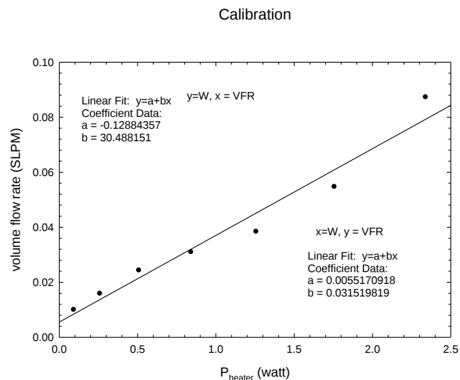
Fig. 8. Calibration curve using the data corrected by the second way. More data at higher heating power values would be necessary.
