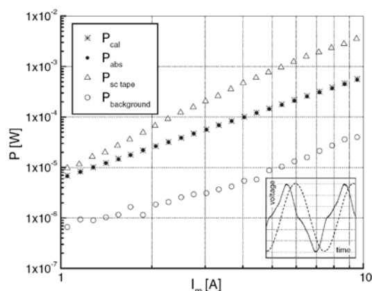
Figure 4. Dependence of the losses on magnet current I_m . P_{cal} —loss of the Cu loop determined as R_{Cu} \times I_m^2 , P_{abs} —loss of the Cu loop evaluated by the proposed method as P_{abs} = \text{Re}(U_{as \text{ loop}}) \times I_m , P_{sc \text{ tape}} —loss of the superconducting tape measured by the proposed method, P_{background} —background loss measured with empty AC field magnet. Inset: waveform of the signal registered with superconducting tape placed in the AC magnet. Dashed curve—current in the AC magnet, full curve—voltage signal measured on anti-serially connected compensation and measurement coil.
