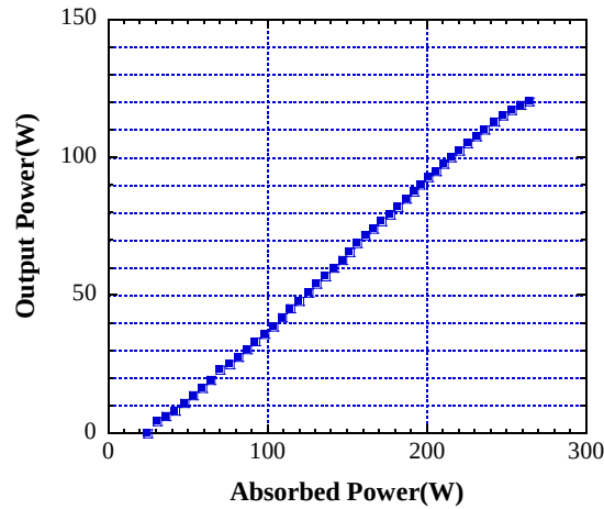
Fig. 4. Relationship between absorbed power and output power for target output from 100 W to 200 W (1st stage).
