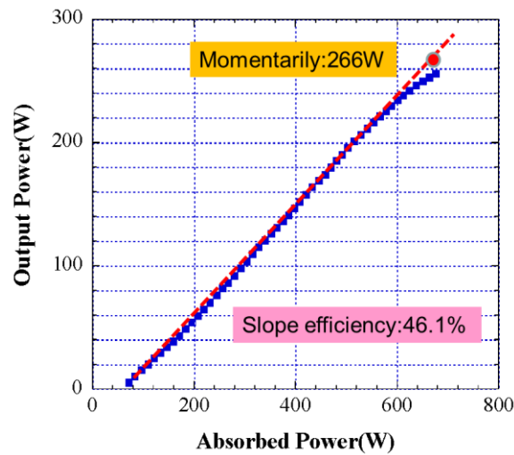
Fig. 5. Relationship between absorbed power and output power for target output from 200 W to 300 W (2nd stage).
