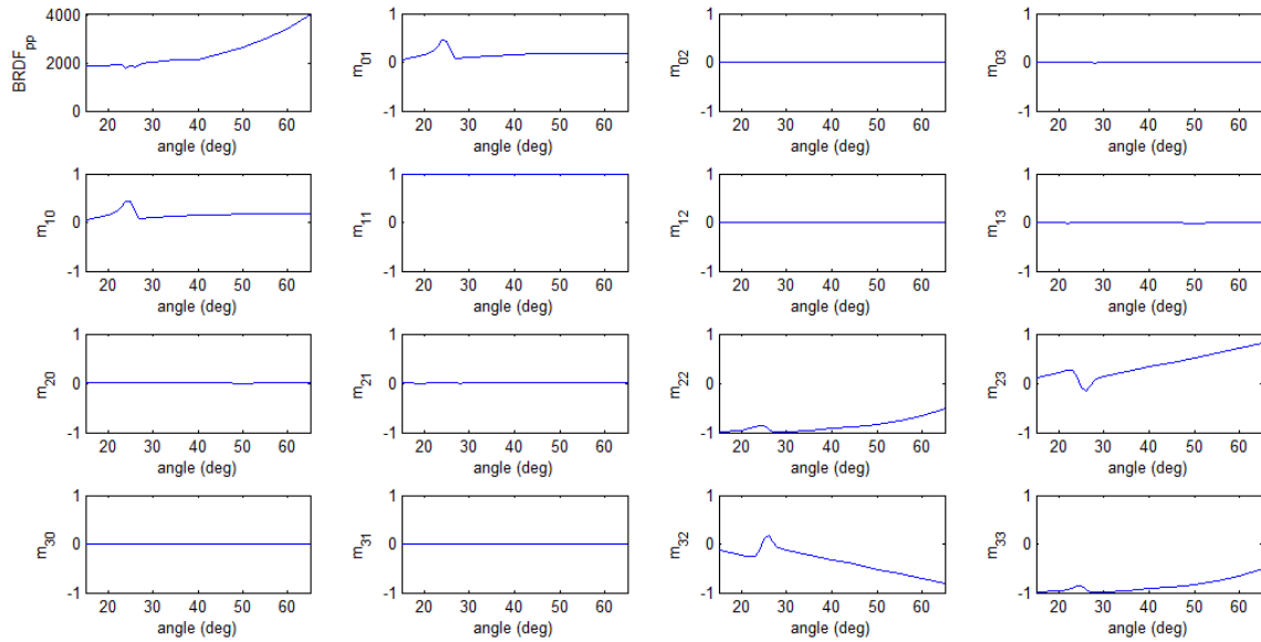
Figure 6-3. Normalized specular reflectance Mm plot for the MMA at 5.0μm.
