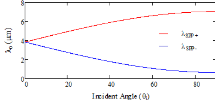
Figure 6-2. Surface plasmon polariton resonance calculated for the MMA, using the material properties of Au at 5.0μm ( \tilde{n} = 3.7 + i0.5 ) [34] and the dielectric ( \tilde{n} = 2.06 + i0.12 ) [17], while the periodic spacing a = 3.2\mu\text{m} .
