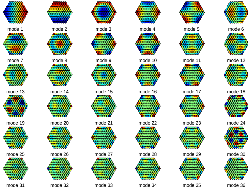
Figure 5 Visualization of Zernike basis reconstructed from Zernike derivative vectors
