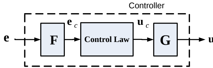
Figure 2 Controller structure for modal control
