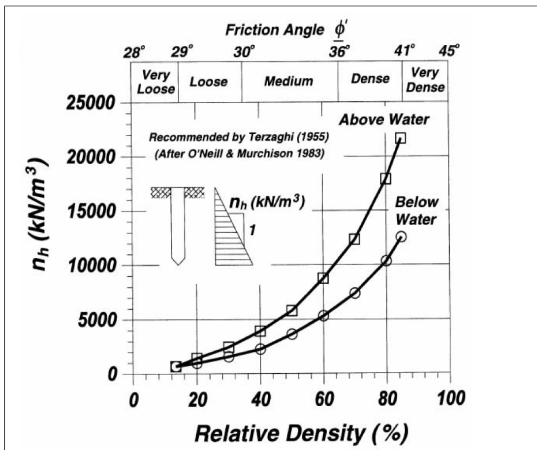
Figure 3-4. Recommended coefficient of subgrade reaction as a function of relative density and friction angle (After ATC-32 1996).
