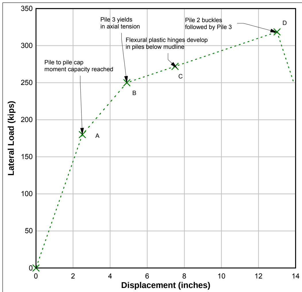
Figure 4-10. Load – displacements plot for batter pile system indicating regions of elastic and inelastic response.
