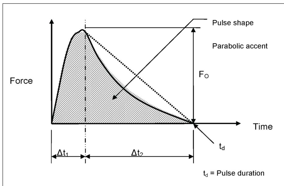
Figure 1-3c. Pulse loading.
