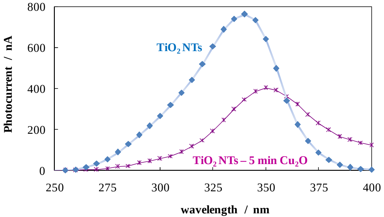
Figure 12 – Raw photocurrent spectra relating to TiO 2 nanotubes soon after annealing and after 5 min of electrodeposition.
