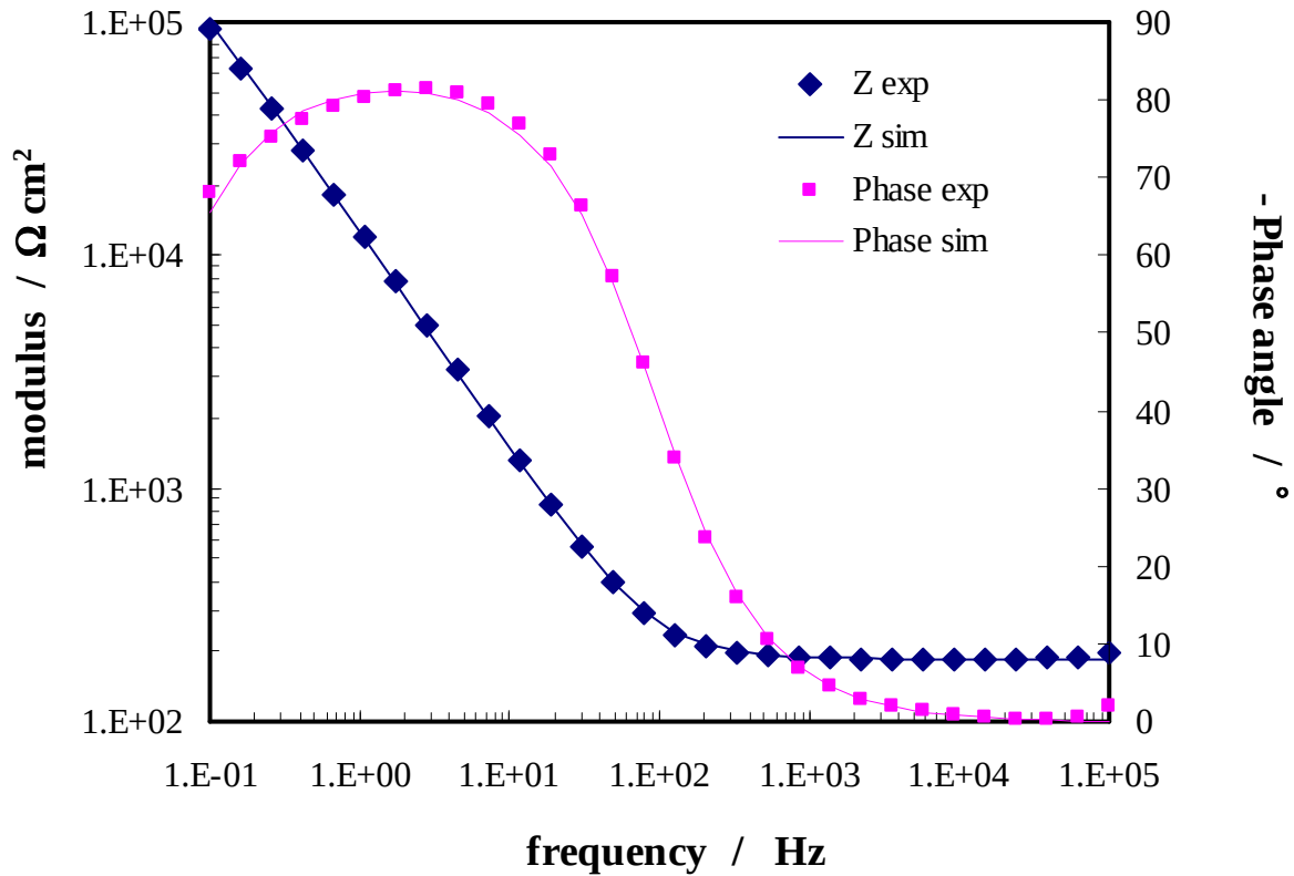
Figure 20 - Measured and simulated impedance and phase angles values relating to the TiO 2 NTs after thermal treatment, recorded by polarizing the electrode of Fig 16 at 0.15 V in 0.1 M Na 2 SO 4 .
