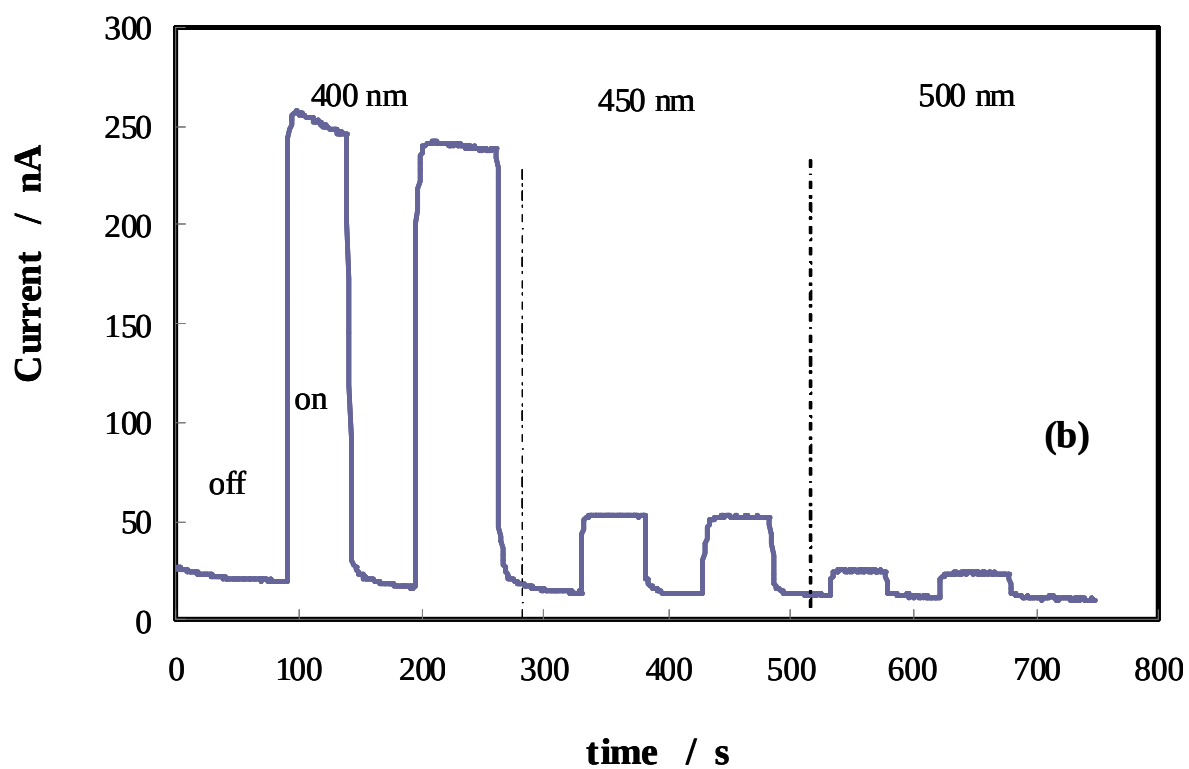
Figure 3 - Current vs time curves relating TiO 2 NTs layer of Fig. 2 recorded at U_E = 0.15 V under dark (off) or light (on) irradiation in 0.1 M Na 2 SO 4 . a) without and b) with the addition of methanol.
