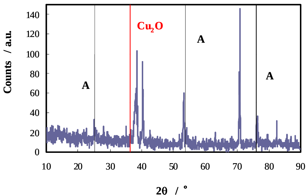
Figure 11 - XRD diffraction pattern relating to \text{TiO}_2 nanotubes after 5 min of electrodeposition. Peaks labelled as A are ascribed to anatase (ICCD card 21-1272), while those not labelled are ascribed to Ti: substrate (ICCD card 44-1294).
