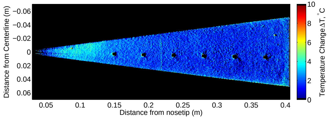
Figure 4. TSP image of the 7^\circ half-angle cone at 0^\circ angle of attack. p_0 = 131 psia, \text{Re}_\infty = 9.9 \times 10^6/\text{m}
