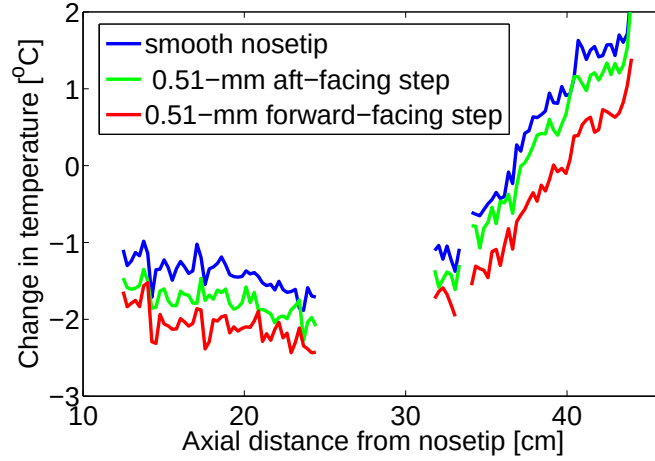
Figure 14. Axial temperature trace on the leeward side of the model for three nosetip configurations. Re = 20 \times 10^6/\text{m} . Gaps in the traces are due to reflections and the lack of optical access between the porthole windows.
