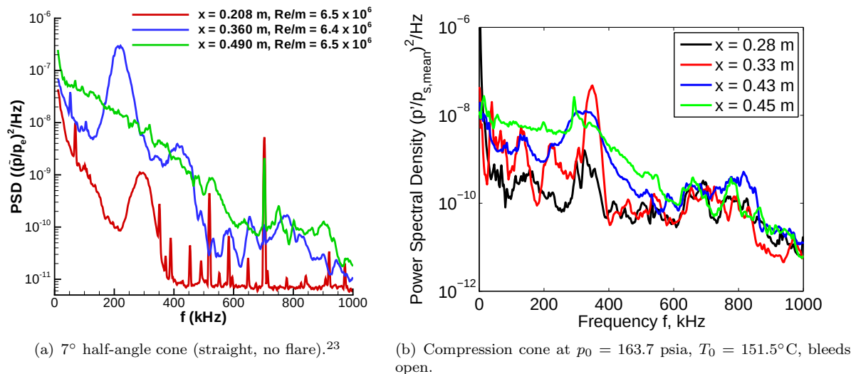
Figure 19. Power spectra of surface pressure fluctuations on two different models.
