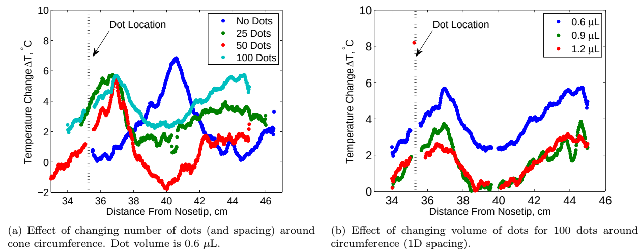
Figure 28. Effects of different dot configurations on streamwise temperature changes.
