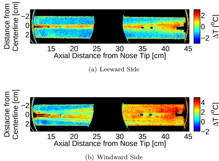
Figure 17. Temperature change behind a 1.5-mm isolated roughness element at Re = 11.2 \times 10^6/\text{m} . Flow from left to right.
