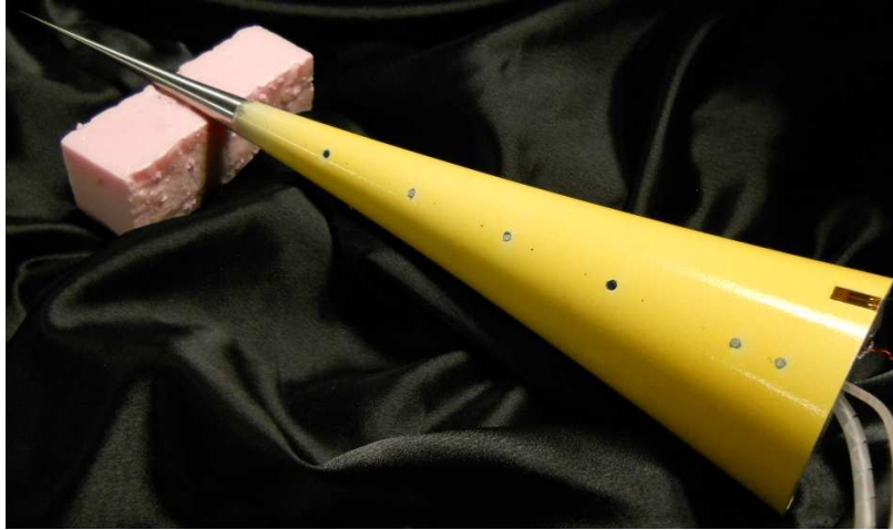
Figure 18. Compression cone model with 0.16-mm nosetip
