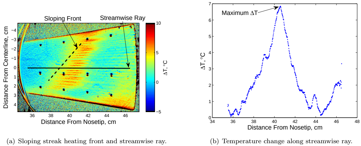
Figure 27. No dots, p_0 = 159.5 \text{ psia} , T_0 = 155.1^\circ \text{ C} .
