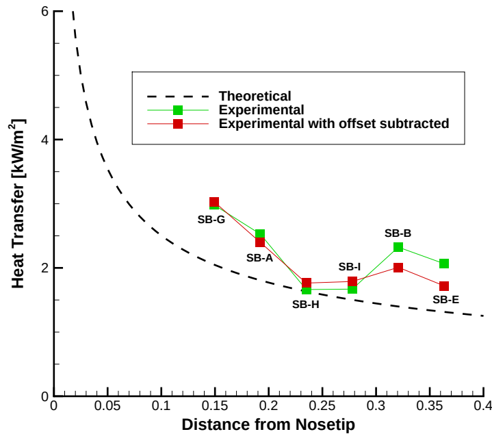
Figure 8. Heat transfer rates with SB gauge positions swapped. p_0 = 131 psia, Re = 9.9 \times 10^6/m . SB-G and SB-H amplified 100 times.
