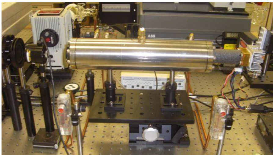
Figure 1. Photograph of the flow-through PA cell.
