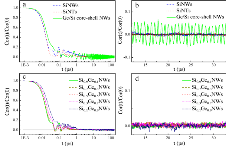
Figure 2. Time dependence of normalized heat current autocorrelation function (HCACF). a, Normalized HCACF for SiNWs (blue dash line), SiNTs (red dot line) and Ge/Si core-shell NWs with L_c/L=0.65 (green solid line). b, Long-time region of a. c, Normalized HCACF for \text{Si}_{1-x}\text{Ge}_x NWs with different doping concentration x . d, Long-time region of c. The black lines in all figures draw the zero axis for reference. Here the super cell size is 16 \times 5 \times 5 and temperature is 300 K.
