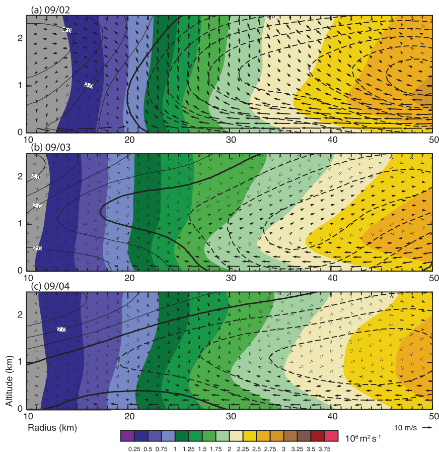
FIG. 10. Hurricane Fabian axisymmetric angular momentum (color), total energy (contours), and secondary circulation (vectors) from 2 to 4 September. The thick contour is 350 \text{ kJ kg}^{-1} ; solid lines and dashed lines indicate values above and below 350 \text{ kJ kg}^{-1} , respectively, with a contour interval of 1 \text{ kJ kg}^{-1} .
