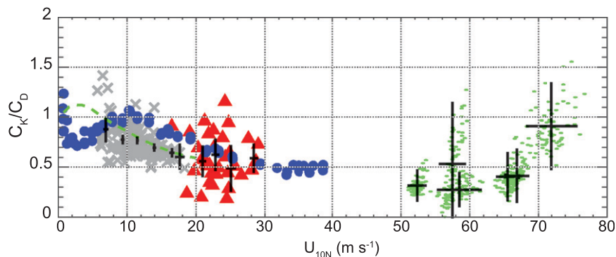
FIG. 21. Wind speed dependence of C_K/C_D from this study (green squares) compared with previous studies. Symbols are as in Fig. 20.
