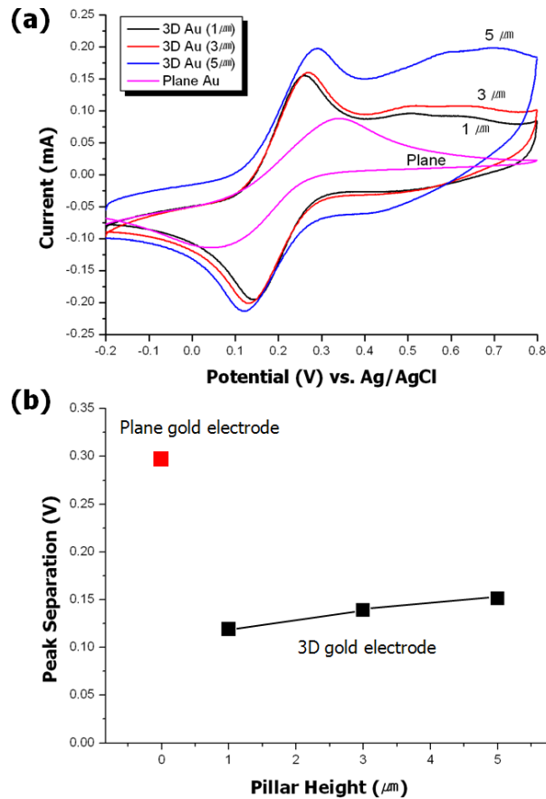
Figure 5. (a) Cyclic voltammograms and (b) the peak to peak separation of 3D gold electrodes with pillars of 1, 3 and 5 μm height and a plane gold electrode.
