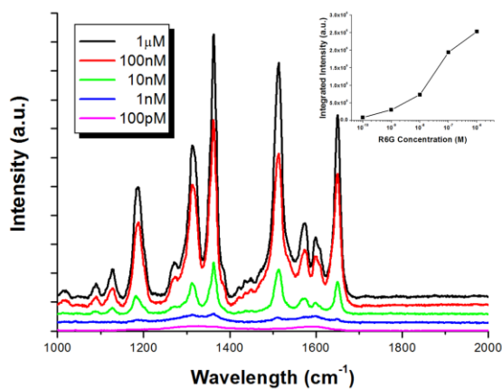
Figure 4. SERS spectra of 3D array of gold nanostructures (3.25 \mu\text{mol}/\text{cm}^2 ) at different R6G concentrations. Each spectrum is the averaged profile of 3 measurements at the different locations. Inserted is the peak intensity at 1362 \text{cm}^{-1} versus R6G concentrations.
