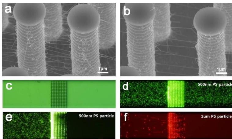
Figure 5. SEM images and optical images of \text{Al}_2\text{O}_3 coated 3D network of SWNTs on (a, c, e) 2.5\mu\text{m} spacing and (b, d, f) 5\mu\text{m} spacing Si pillar templates in microfluidic channel. (c) Microscopic image of Si micropillar in microfluidic channel. And fluorescent microscopic images of (d) passing 500 nm green-PS particles through 3D networks on 5\mu\text{m} spacing Si pillar template, (e) filtered 500 nm green-PS particles by 3D networks on 2.5\mu\text{m} spacing template, and (f) filtered 1\mu\text{m} red-PS particles by 3D networks on 5\mu\text{m} spacing template.
