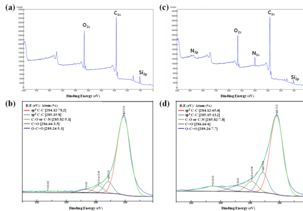
Figure 7. XPS spectra of (a-b) as-synthesized SWCNTs and (c-d) after NH 3 plasma treatment.
