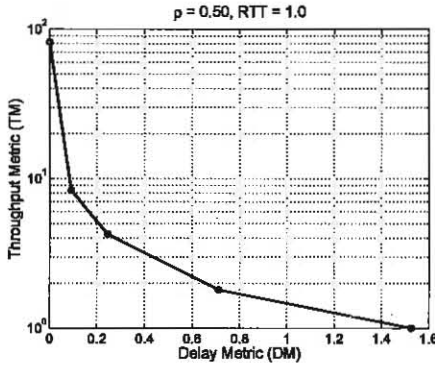
Fig. 4. Delay Throughput Tradeoff
