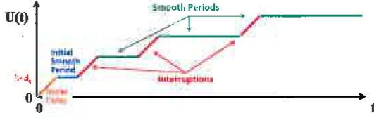
Fig. 5. User perceived delay.
