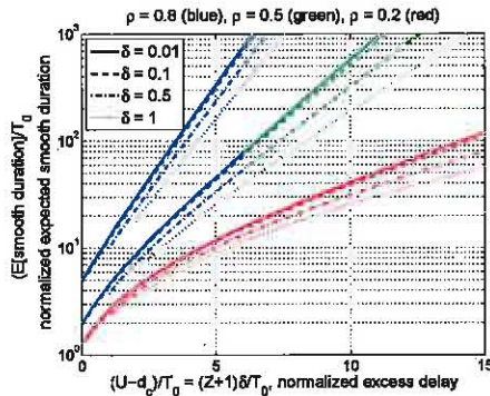
Fig. 6. Expected Smooth Duration.
