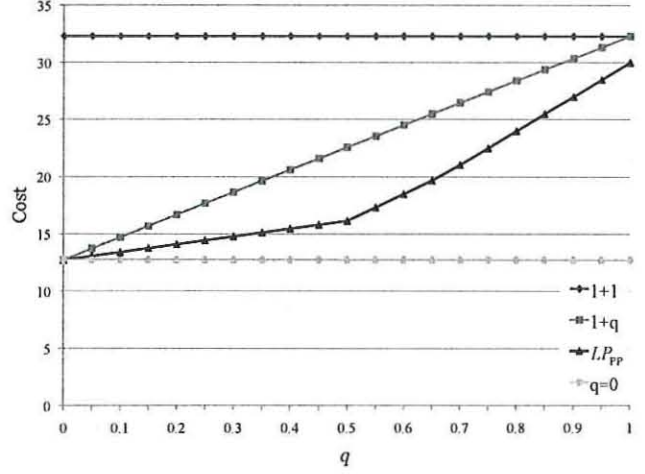
Fig. 3: Capacity Cost vs. q
