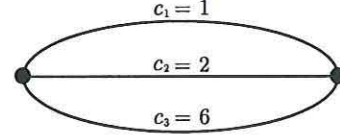
Fig. 4: Two-node network with link costs
