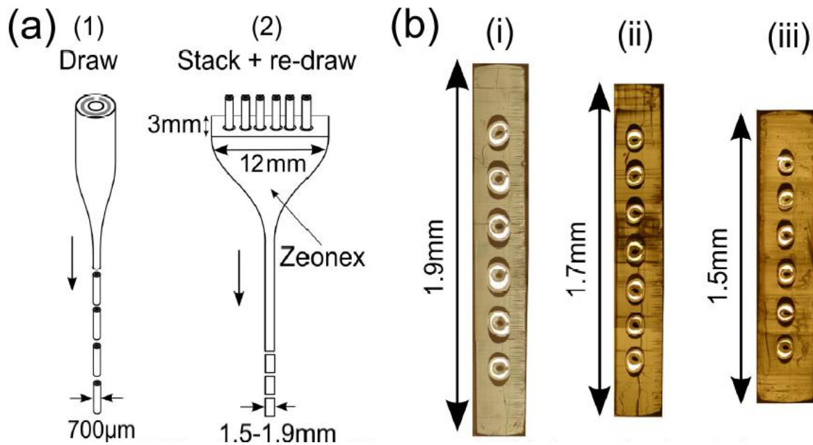
Figure 1: from Ref. 1: Schematic of the stack-and-draw metamaterial fabrication procedure. A cm-sized preform similar to that presented in Fig. 1(a) is drawn down to a 700\ \mu\text{m} fiber and cut into 30 cm pieces. Each piece is inserted into the six holes of a 12 \times 3\ \text{mm}^2 rectangular Zeonex preform. This entire structure is re-drawn down to rectangular fibers of 1.5-1.9 mm. (b) Optical microscope image of the cross section of (i) 1.9 mm, (ii) 1.7 mm and (iii) 1.5 mm wide rectangular fiber, containing six slotted resonators. Note that fibers (i) and (ii) have been polished on the sides.
