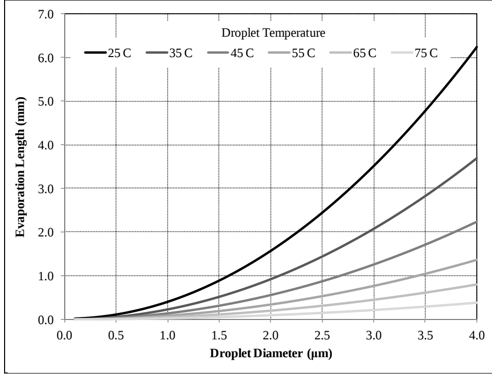
Figure 3. Evaporation length versus ethanol droplet diameter droplet temperatures ranging from room temperature to just below boiling and within air at room temperature.
