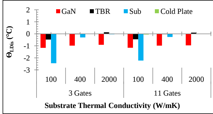
Figure 30. Layer temperature rise discrepancy as a function of substrate thermal conductivity and gate number (table 1 parameters).
