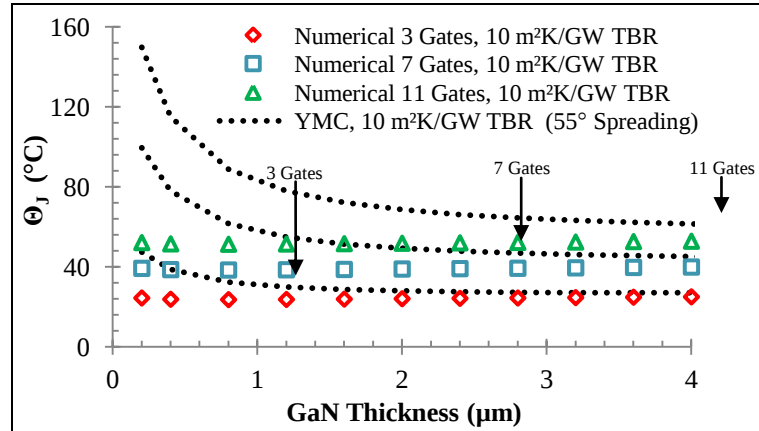
Figure 4. Junction temperature as a function of GaN thickness and gate number for numerical and YMC models (10 \text{m}^2\text{K}/\text{GW} TBR and table 1 parameters).
