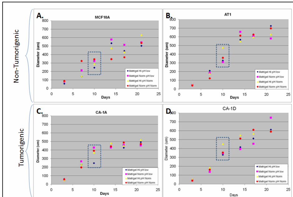
Figure 5. MCF-10A, -AT1, -CA1a and -10 CA1d cell line variants were cultured in the presence of standard (~3 mg/ml Matrigel) or High Concentration Basement Membrane (20 mg/ml) under either neutral or low pH media conditions. Cells were maintained in either standard pH (7.4) media, or low pH media (DMEM/F12 standard media + 10mM MES pH 6.6) throughout the 21 day culture period. Shown are average diameter of mammospheres at 3, 7, 10, 14, 17 and 21 days of culture. Blue: High Matrigel/Low pH; Pink: standard Matrigel/Low pH; Yellow: High Matrigel/Neutral pH; Red: Standard Matrigel/Neutral pH.
