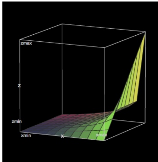
Figure 2. p^{nw*} Under Example 2.2.2: Constant Absolute Risk-Aversion Utility Function
