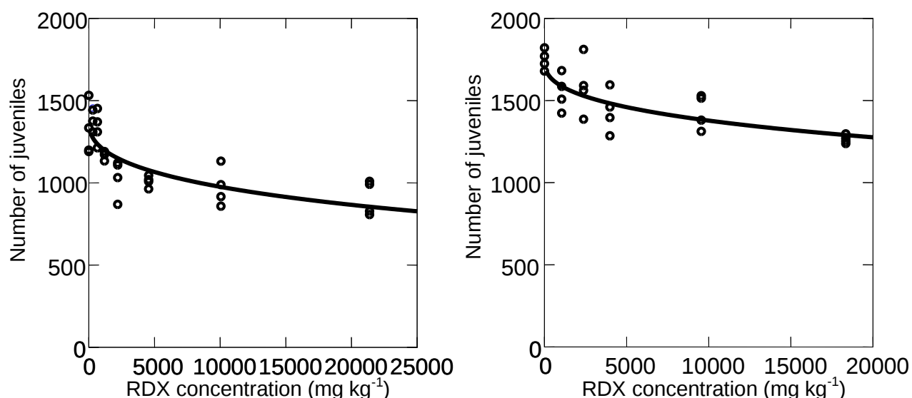
Figure 8. Effects of RDX FA (left) or W-A (right) in SSL soil on production of juveniles by E. crypticus . Data were reported initially in Kuperman et al. (2004a) and are included in this report for convenience of comparison with other soils.
