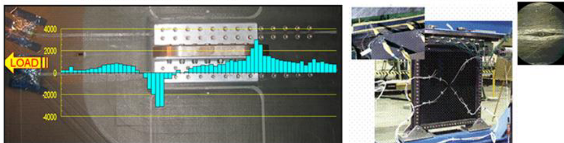
Figure 2-4: FBG Sensors Embedded in Composite Structures. Strain measurements from FBGs embedded under bolted joint on the composite crew module panel (left), and fiber optic sensors embedded in 2 ft by 2 ft shear panel (right).
