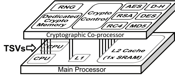
Fig. 4: Our proposed 3-D cryptographic co-processor, complete with dedicated memory for crypto keys and state.
