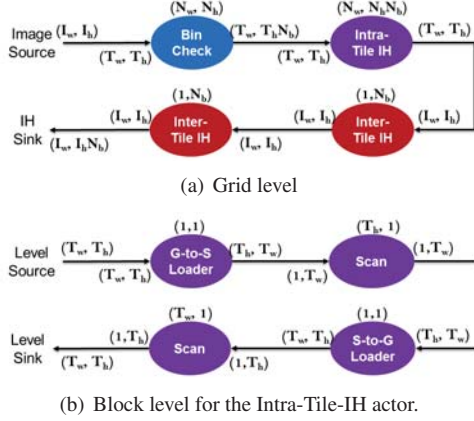
Fig. 4. Hierarchical dataflow graphs for cross-weave TIH.
