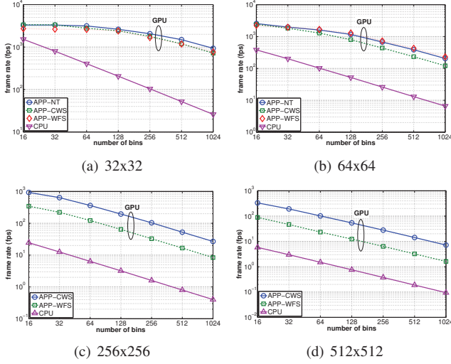
Fig. 5. Performance comparisons for different image sizes.
