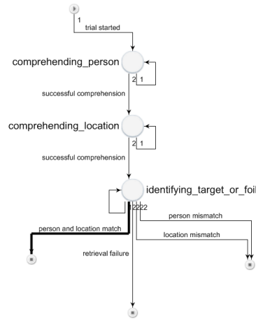
Figure 7. EFSM representing behavior that comprehends a person, comprehends a location, and then identifies a trial as a target or a foil.
