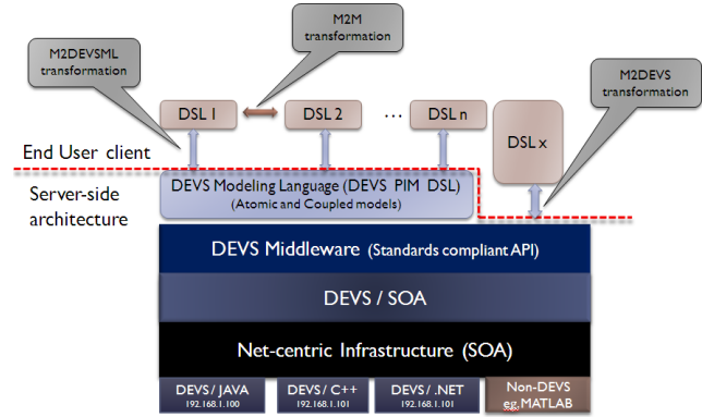
Figure 4. DEVSM 2.0 stack employing M2M and M2DEVS transformations for Model and simulator transparency
