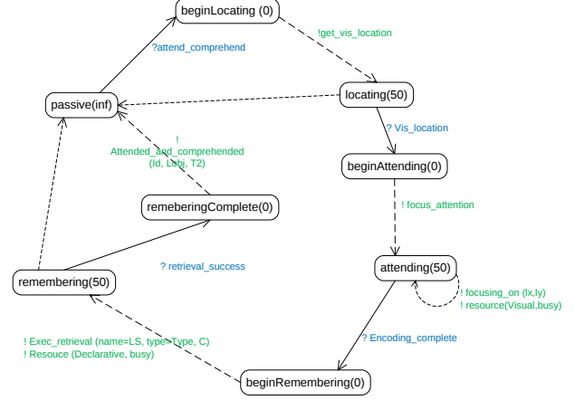
Figure 9. FDDEVS state machine for attend_and_comprehend
