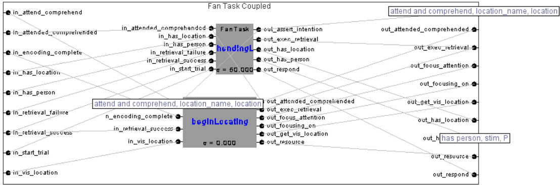
Figure 10. Fan Task Coupled Model
