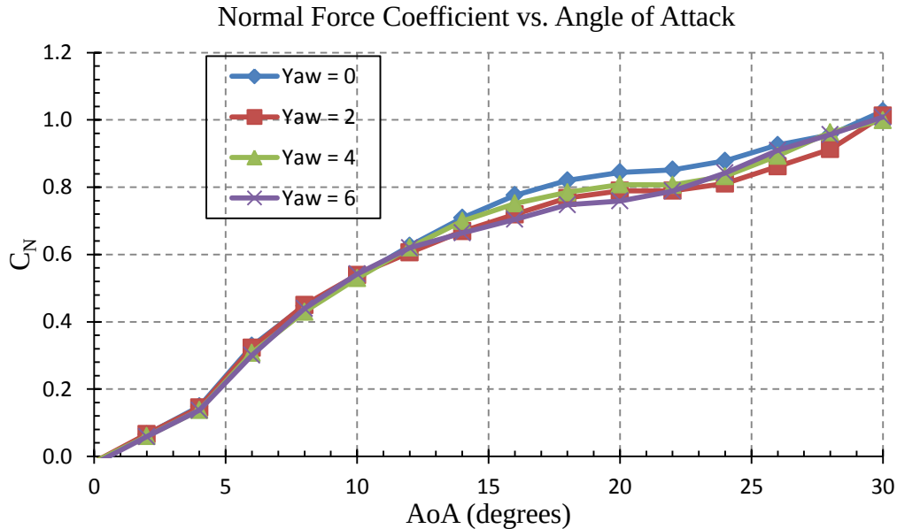
Figure 23. Yaw Angle Effects on Normal Force Coefficient, Steady Flow, Re = 2.3 \times 10^4 .
