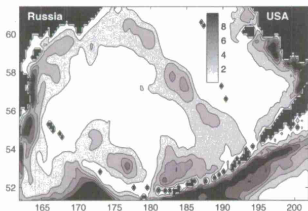
Fig. 8 Horizontal distribution of the eddy kinetic energy ( \text{J/m}^3 ) averaged in the 0–300 m water column
