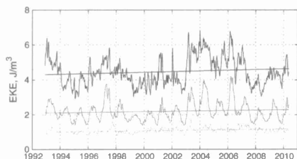
Fig. 9 Evolution of the BS eddy kinetic energy at (from top to bottom) 20, 187 and 900 m averaged for the domain shown in Fig. 1. Thin straight lines show the long-term trends
