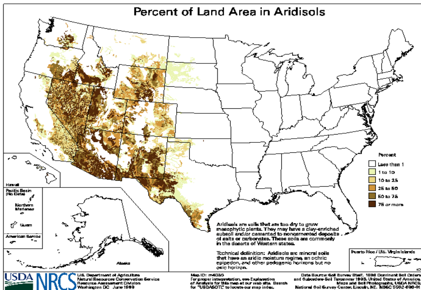
Figure 10. The above figure from the http://www.cals.uidaho.edu/soilorders/percentarid.gif shows the distribution of Aridisols in the US and includes areas of the ASD collection sites and AVIRIS imaged areas. Knowing what soils are present in an area will be helpful in making predictions about how soil properties will respond to surface disturbances, which can in turn aid in tracking those disturbances consistently (Lammers, 1991; Whitford, 2002).
