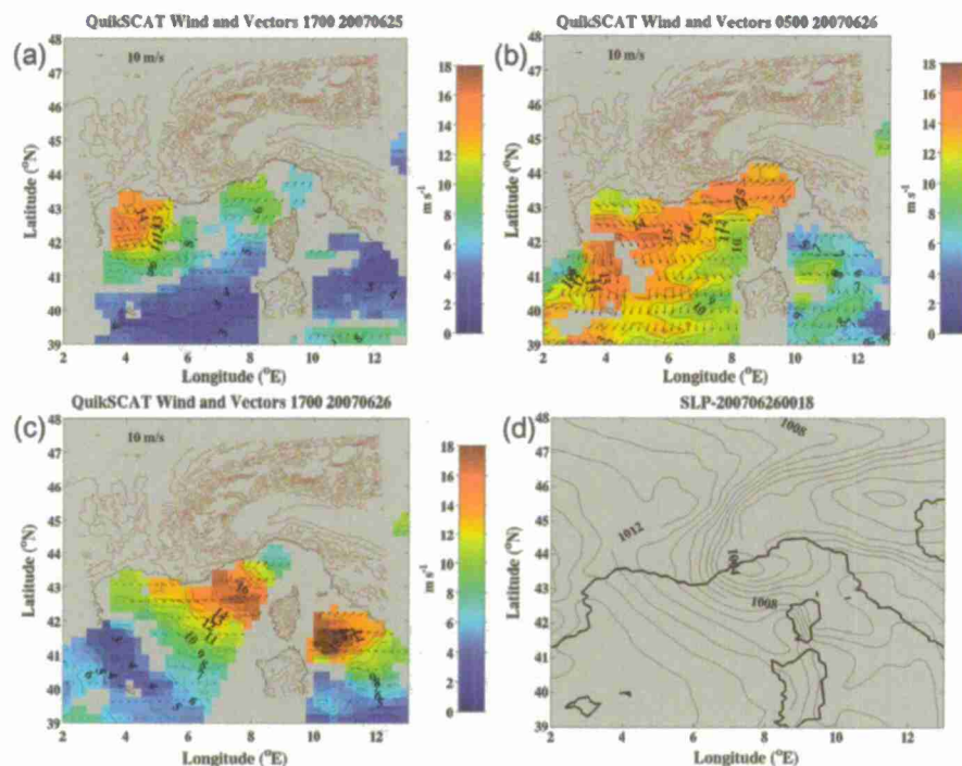
Fig. 2. Near-surface winds and sea level pressure during the Mistral. (a–c) 10 m neutral winds from QuikSCAT swaths at (a) 25th June, 2007, 1700Z, (b) 26th June 0500Z, and (c) 26th June 1700Z. Here colors show the wind speed and the velocity vectors are referenced to the 10 \text{ m s}^{-1} scale at top left. The brown contours over land are land topography at 500 m intervals. (d) Sea level pressure field (hPa) from nest 2 of the atmospheric model at 1800Z, 26th June 2007. Contour Interval is 1 hPa. (For interpretation of the references to color in this figure legend, the reader is referred to the web version of this article.)
