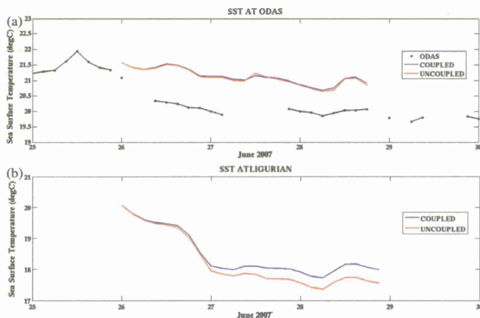
Fig. 6. SST evolution in the inner ocean model nest. (a) The 'ODAS' location, 9°9.8'E, 43°47.36'N (9.16°E, 47.79°N), and (b) in the central Ligurian Sea (8.00°E, 43.00°N). Curves show results from the coupled (blue) and uncoupled (red) runs, and in (a) at ODAS the observations are shown in black with some SST data missing. (For interpretation of the references to color in this figure legend, the reader is referred to the web version of this article.)
