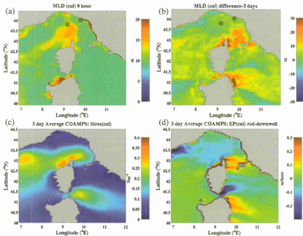
Fig. 10. (a) Initial mixed layer depth (m) from the coupled model. (b) Mixed layer depth change (m) over 69 h from coupled run (c) 3 day average of wind stress ( \text{Nm}^{-2} ) repeated from Fig. 9b. (d) The 3 day average of negated Ekman pumping velocity ( \text{m h}^{-1} , positive downwards convention such that red areas denote downwelling).
