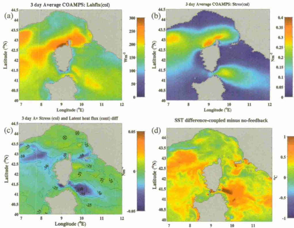
Fig. 9. Three-day averages (26–28 June) from the coupled model of (a) surface latent heat flux \text{Wm}^{-2} and (b) surface stress \text{Nm}^{-2} . (c) shows the difference of 3-day average latent heat flux ( \text{Wm}^{-2} contour) and stress (color) between the coupled run minus the uncoupled atmosphere run, (d) difference in the SST final state between the coupled run and uncoupled ocean run.
