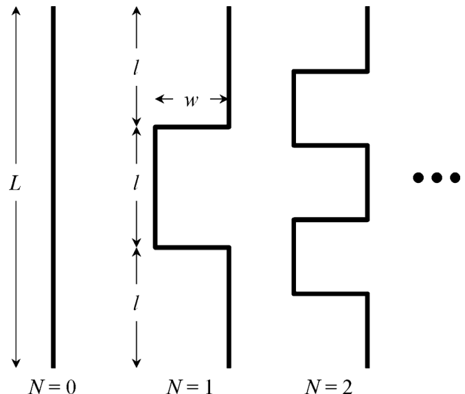
Fig. 1. One arm of an SLDA compared to one arm of MLDAs with increasing numbers of bends N . For each meandered dipole arm, all horizontal segments are of equal length w , and all vertical segments are of equal length l . Dimensions and resonant frequency for L = 30 cm and cases up to N = 6 meanders are shown in Table I.
