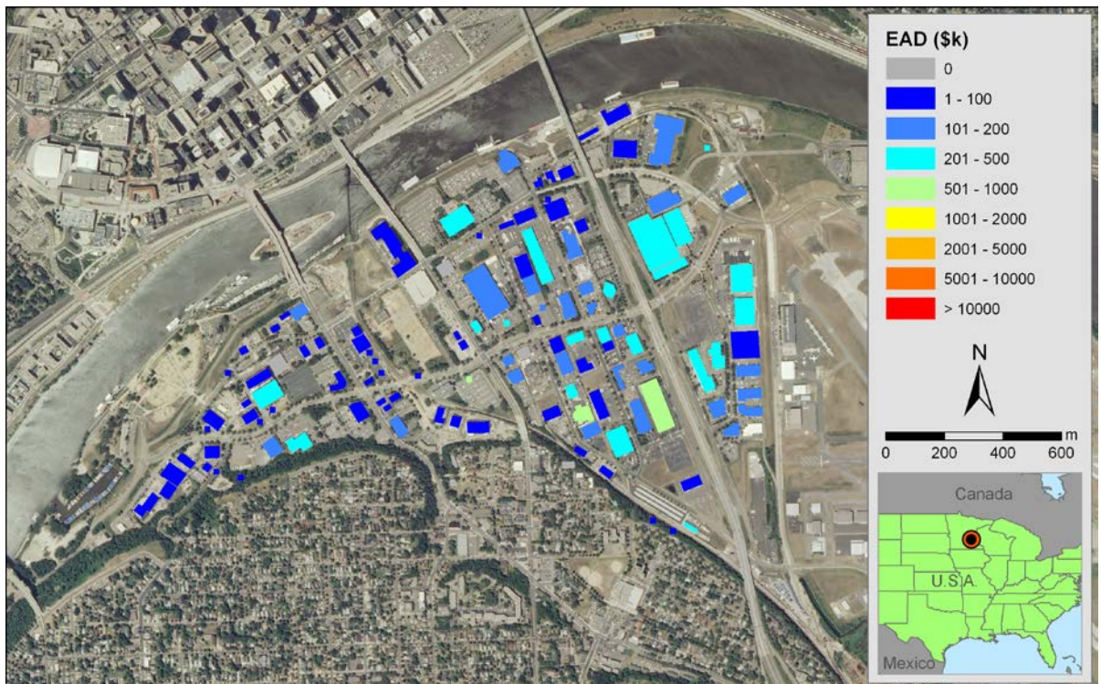
Figure 3.14 Spatial distribution of residual floodplain risk, EAD ($k), reference case (existing situation)
