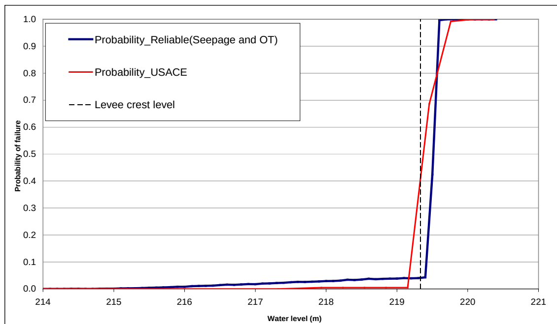
Figure 3.4a Reach 1 Fragility curves from RELIABLE and USACE 2011
