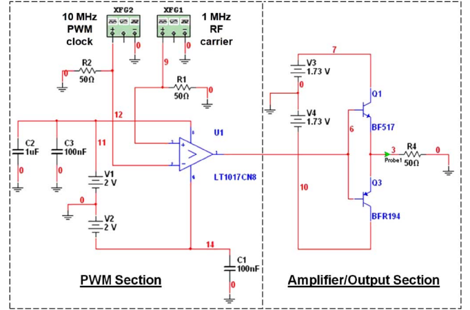
Fig. 5. Schematic of complete DDA system as represented in National Instruments' Multisim Circuit Design program. Transmit and receive antenna models from Fig. 4 are substituted for the 50-Ω resistor R_4 in the simulation of the full DDA system.
